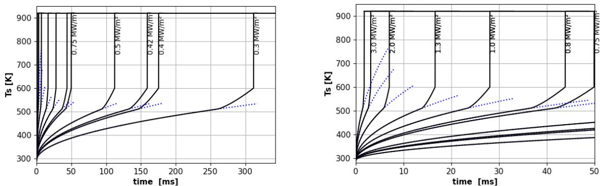
Figure 8. Simulated surface temperature evolutions determined by the simple model for laser power density ranging from 0.3 to 4.0 MW/m 2 .
