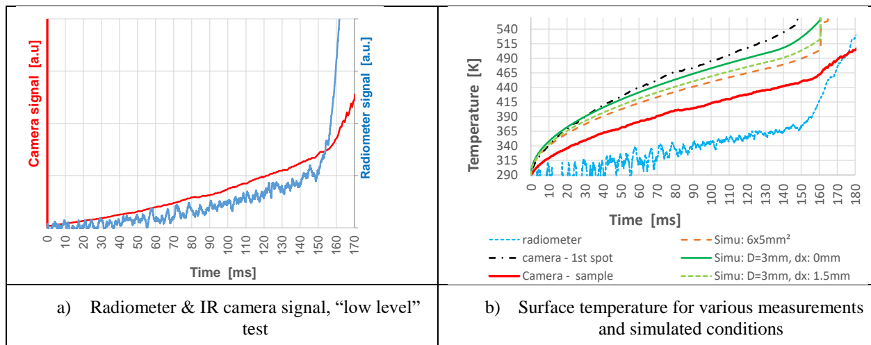
Figure 18. Signal and surface temperature for the "low level" ignition test.
