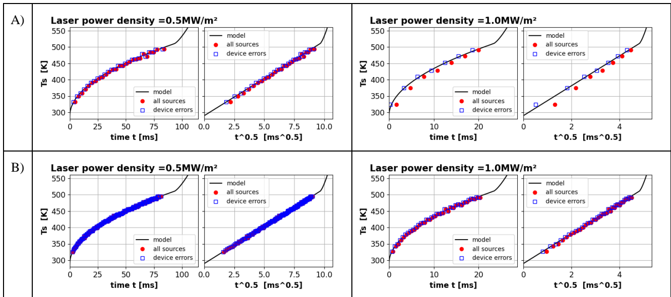
Figure 11. Example of random draws for laser power density 0.5 and 1.0 MW/m 2 .
