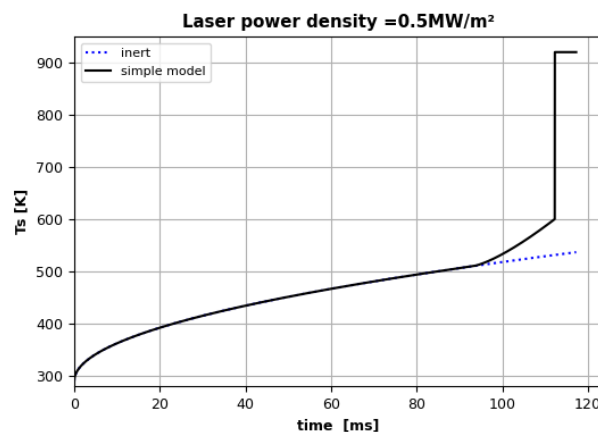
Figure 1. Example of simulated surface temperature computed by the simple demonstration model. Blue dots: inert heating. Black line: complete model.
