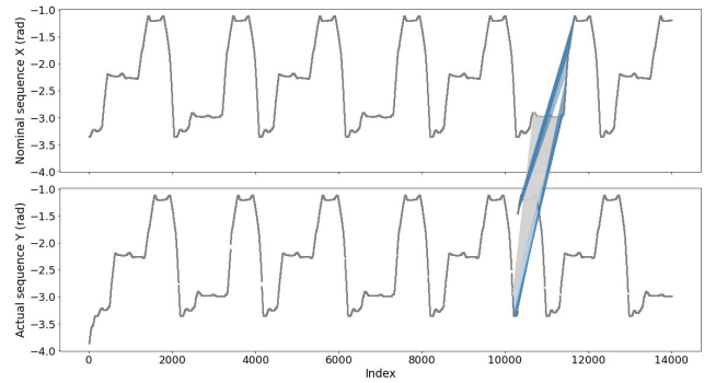
Figure 10: Signals used for Experiment 2. X (above), Y (below), and some S-DTW warping path pairs (in gray and blue).
