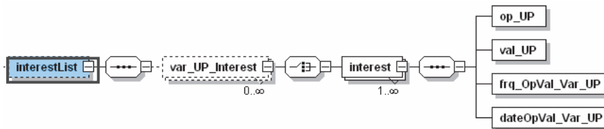
Fig. 1.b. The user's interests in XML Schema
