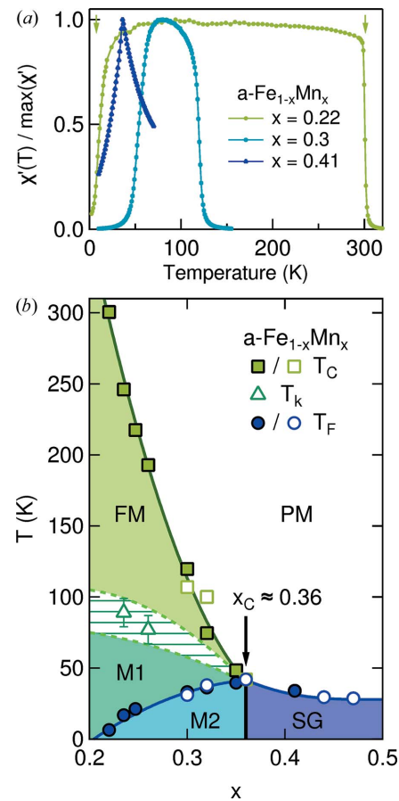
Figure 2 (a) The zero-field a.c. susceptibility of a- Fe_{1-x}Mn_x for x = 0.22, 0.3 and 0.41 , recorded under an a.c. field of 10 Oe amplitude and 1 kHz frequency [data taken from Martin et al. (2021)]. The Curie ( T_C ) and freezing ( T_F ) temperatures are defined as the high- and low-temperature inflection points, respectively (as shown by the arrows for x = 0.22 ). (b) A phase diagram reconstructed from such data. T_C and T_F values are from Martin et al. (2021) (solid symbols) and Yeshurun et al. (1980) (empty symbols). T_k is determined from Mössbauer spectroscopy and muon spin relaxation ( \mu SR) (Mirebeau et al. , 1986, 1997).
