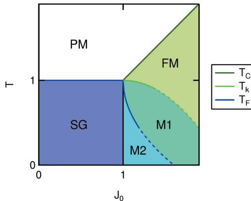
Figure 1 Mean-field phase diagram for a bond-disordered ferromagnet calculated using the model of Gabay & Toulouse (1981) for Heisenberg spins. The various transition temperatures are indicated for further reference. Dashed lines illustrate the fact that the obtained M2 \leftrightarrow M1 and M1 \leftrightarrow FM transition lines are only exact close to the multicritical point ( i.e. for J_0 \gtrsim 1 ).
