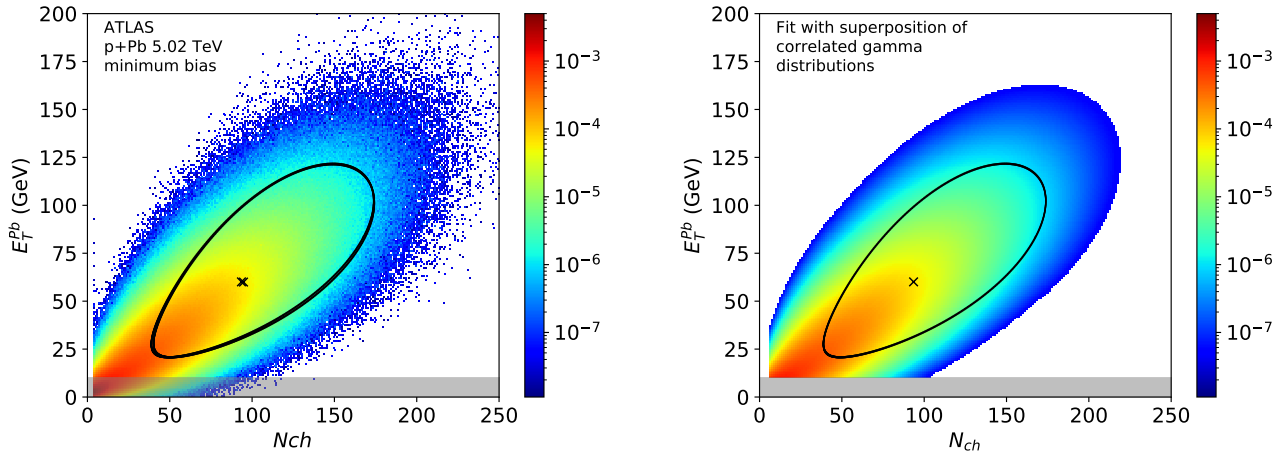
FIG. 5. (Color online) Joint probability distribution of N_{ch} and E_T^{Pb} in minimum-bias p+Pb collisions at \sqrt{s_{NN}} = 5.02 TeV. Left: ATLAS data [31]. Two lines are drawn, which almost coincide, and correspond to the 90% area of b = 0 collisions given by the Bayesian reconstruction for two different initializations of the fit, as in Fig. 4. Right: fit using Eq. (13) for one specific initialization. We have applied the cuts N_{ch} \geq 6 and E_T^{Pb} > 10 GeV, and the excluded range is shown as a shaded area. In the right panel, the cut between the colored region and the white region has been placed arbitrarily (due to the various triggers used by ATLAS, the rule of one event per bin used in previous plots was ambiguous).
