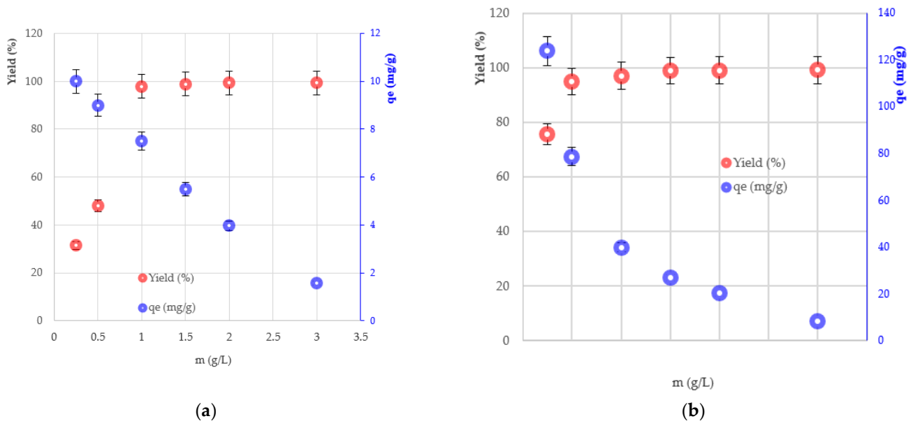
Figure 4. Effect of adsorbent dosage on the percentage of removal and amount of dyes adsorbed on 4AZW: (a) MB; (b) MG ( C_0(\text{MB}) = 8 \text{ mg/L} , C_0(\text{MG}) = 41 \text{ mg/L} , contact time 70 min, T = 25 \pm 1 \text{ }^\circ\text{C} and unadjusted pH).
