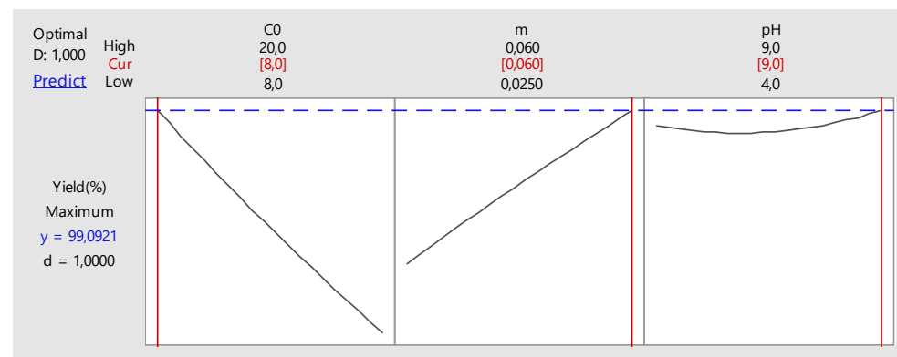
Figure 10. Diagrammatic optimization of MB removal parameters.
