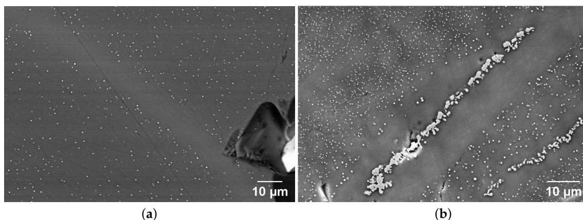
Figure 3. SEM imaging of (a) red sample 29 in AsB detection and (b) orange sample 70 in SE2 detection.
