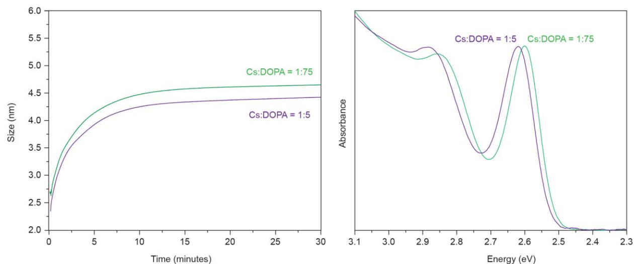
Fig. S4. Experiments with the high excess of DOPA acid, with keeping all other reaction conditions fixed, demonstrating that excess DOPA does not influence the growth of CsPbBr 3 .
