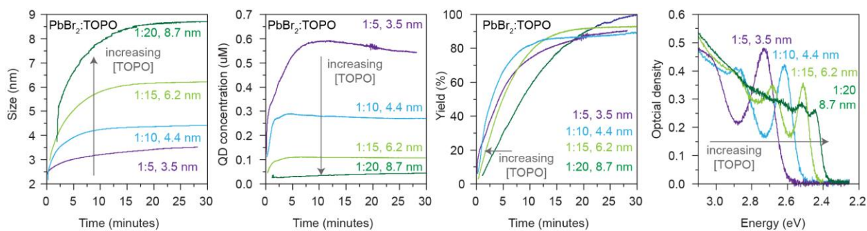
Fig. S31. Further details, including size, QD concentration, reaction yield and final optical absorption spectra of differently sized \text{CsPbBr}_3 QDs obtained with various concentrations of TOPO.
