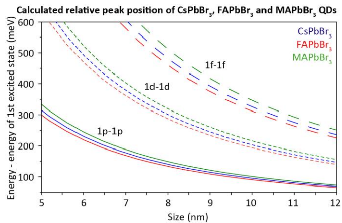
Fig. S42. Calculated relative absorption transition peak position of CsPbBr 3 , FAPbBr 3 and MAPbBr 3 QDs as function of QD size, demonstrating relative peak position is independent of the A-site cation.
