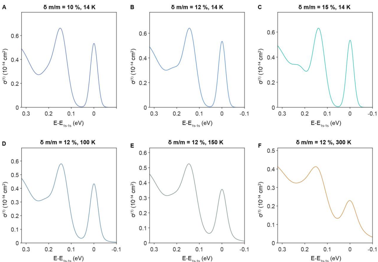
Fig. S38. Theoretical absorption spectra for CsPbBr 3 with the splitting in the 1p-1p transition at low temperature. The QD size is L = 7.3 nm for which the size dispersion was taken to be \delta_{size} = 8\% . The aspect ratio b , as discussed in supplementary text, was fixed 1.03 as obtained from SAXS measurements. The widths of the 1p states were set to be 75% of the estimated line shape outlined in supplementary text for the splitting to be visible. As the mass variation \delta m/m increases from 10% to 12% and then 15%, the separation between the 1p-1p peaks grows bigger as manifested in the spectra in panels a-c at T = 14 K. Fixing \delta m/m = 12\% , the calculations with increasing temperature where T = 100 K, 150 K and 300 K shows that the p-state splitting is no longer observable at room temperature due to thermal broadening.
