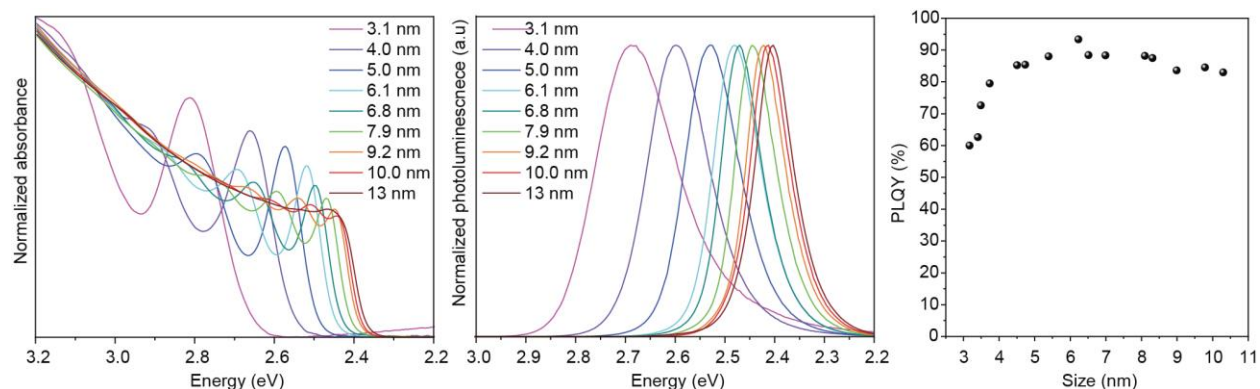
Fig. S16. Additional absorption and PL spectra of purified CsPbBr 3 QDs as well as their respective PLQYs.
