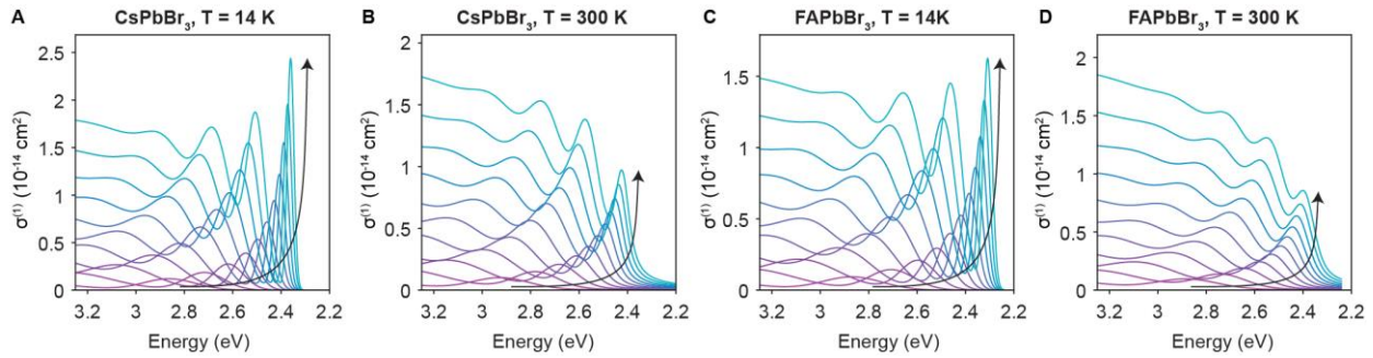
Fig. S32. Theoretical one-photon absorption cross-section \sigma^{(1)} ( 10^{-14} \text{cm}^2 ) versus energy (eV) for different sizes using spherical k.p model. The direction of increasing size, where L = 3.0 - 8.0 nm with size step equal to 0.5 nm, is indicated by a black arrow. A and B , CsPbBr 3 , C and D , FAPbBr 3 . The absorption spectra were calculated at 14 K (panels A and C ) and at 300 K (panels B and D ). The broadening parameters used for CsPbBr 3 and FAPbBr 3 QDs are discussed in Supplementary Text.
