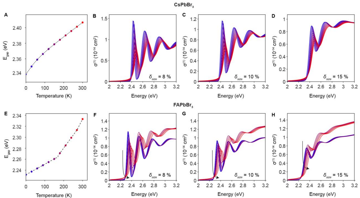
Fig. S33. Temperature dependence of one-photon absorption cross-section spectrum \sigma^{(1)} ( 10^{-14} \text{cm}^2 ) versus energy (eV) in spherical k.p model. A-D , CsPbBr 3 , E-H , FAPbBr 3 . QD size is L = 7.0 nm for both cations. The arrows denote direction of increasing temperature. Each calculated spectrum corresponds to the temperature represented by each dot on the leftmost panels. The size dispersion \delta_{size} is 8%, 10% and 15% from left to right (panels B to D for CsPbBr 3 , panels F to H for FAPbBr 3 ). For CsPbBr 3 , the temperature-dependent electronic band gap is modelled as in Ref (63). Using A_{linear} = 0.339 meV/K,(63) and E_{LO} = 16 meV,(53) the choice of A_{LO} = 30 meV correctly reproduces the absorption band gap of CsPbBr 3 as measured by Yang et al (50). The change of E_{gap} of FAPbBr 3 versus temperature was fitted using linear function for the data from Wang et al (64).
