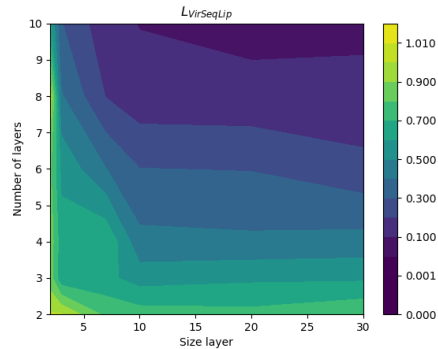
Fig. 3: Computation of the Lipschitz constant using the seqLip algorithm for different depths (y axis) and different layer size (x axis) with numpy optimizer.
