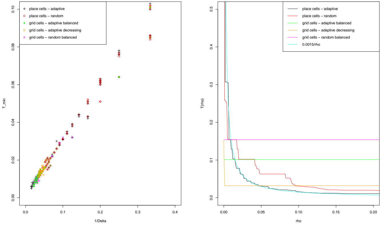
Figure 2: Discrimination time as a function of \Delta_{s_1, s_2}^f and \rho . On the left, T_{min}(f, s_1, s_2, \alpha) as a function of 1/\Delta_{s, s'}^f for the 5 different codes. On the right, T_{min}(f, \rho, \alpha) as a function of \rho for the 5 different codes.
