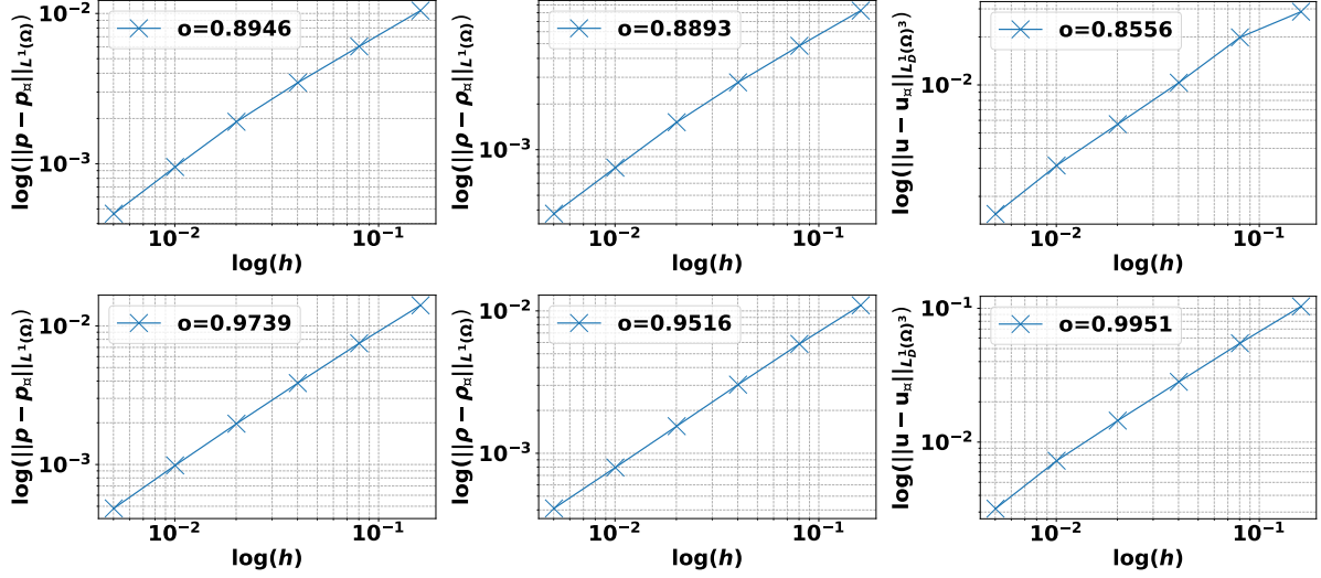
FIGURE 11. Convergence rate for the problem of a shock with reflexive boundary condition on a sequence of prismatic meshes. From left to right : pressure in L^1(\Omega) norm, density in L^1(\Omega) norm, velocity in discrete L^1(\Omega)^d norm. From top to bottom : error at time t = 0.003 , errors at time t = 0.015 .
