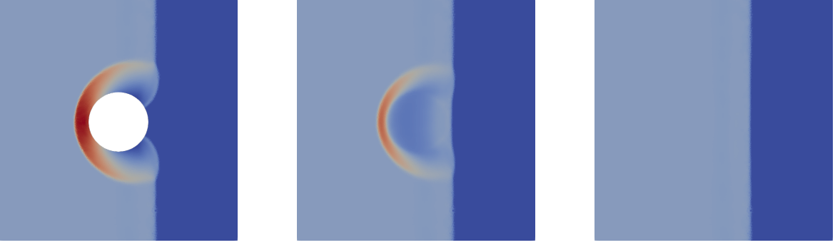
FIGURE 9. Density for the problem of the shock on a column on a prismatic mesh, at time t = 0.026 . From left to right : cut at z = 0.01 , cut at z = 0.31 and cut at z = 0.4 .
