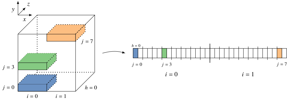
Figure 2. One-dimensional structure array of the component grid \Omega_{h_1} , \mathbf{l} = (1, 3, 1) . Indexes ranges from i = 0, 1 , j = 0, 7 , h = 0, 1 . The cells of the three-dimensional grid are arranged in a one-dimensional array where the z -dimension is the fast axis and the x -dimension is the slow axis.
