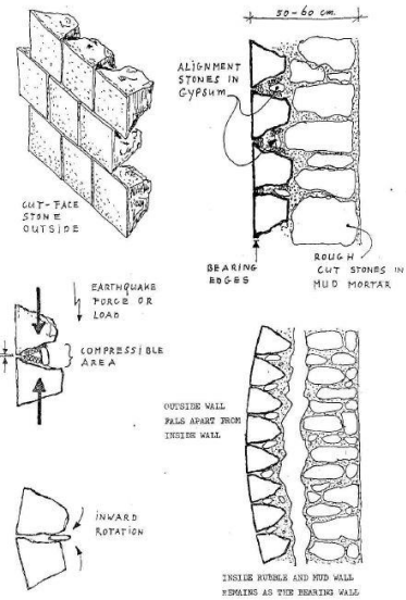
Study of stone wall weakness to earthquake, stone are squard – source Sjoerd Nienhuys 1984
