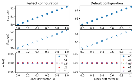
Figure 19: Exp R.4: Guard bands (upper panels) and optimal offsets (bottom panel) versus clock nonideality factor x , where \Delta = x\mu\text{s} , \eta = 2x\text{ns} , \rho = 1+10^{-4}x (Ring topology).
