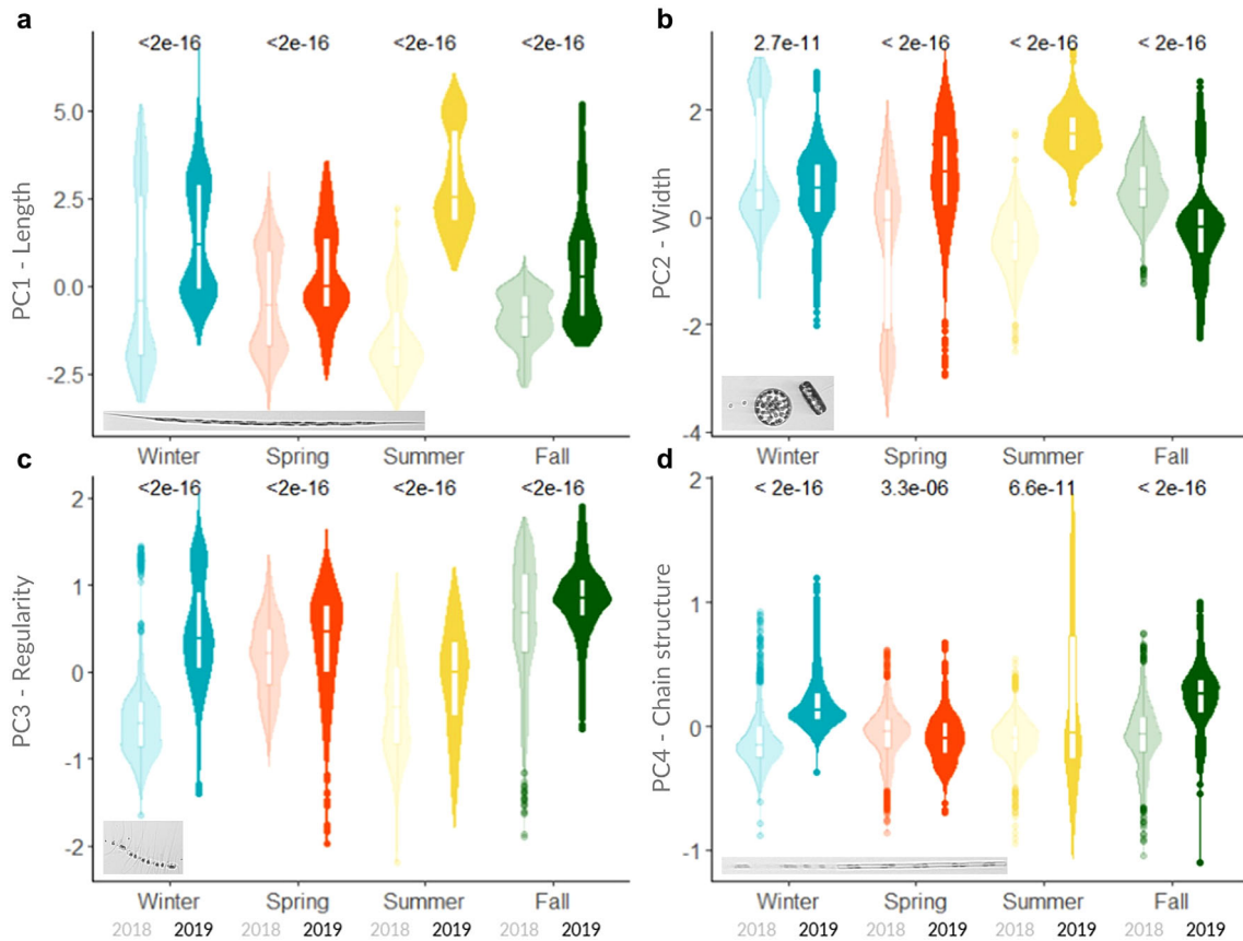
Fig. 7. Distribution of morphological traits per season and per year. The distributions are colored by season (winter in blue, spring in red, summer in yellow and fall in green) and contrasted per year (lighter in 2018 and darker in 2019) for (a) the length, (b) the width, (c) the shape regularity, and (d) the chain structure. The p -value of a Wilcoxon test comparing the 2018 and 2019 means for each season is displayed on top of the violin plots. The year 2018 refers to data between November 2017 and September 2018 and the year 2019 refers to data between October 2018 and October 2019.
