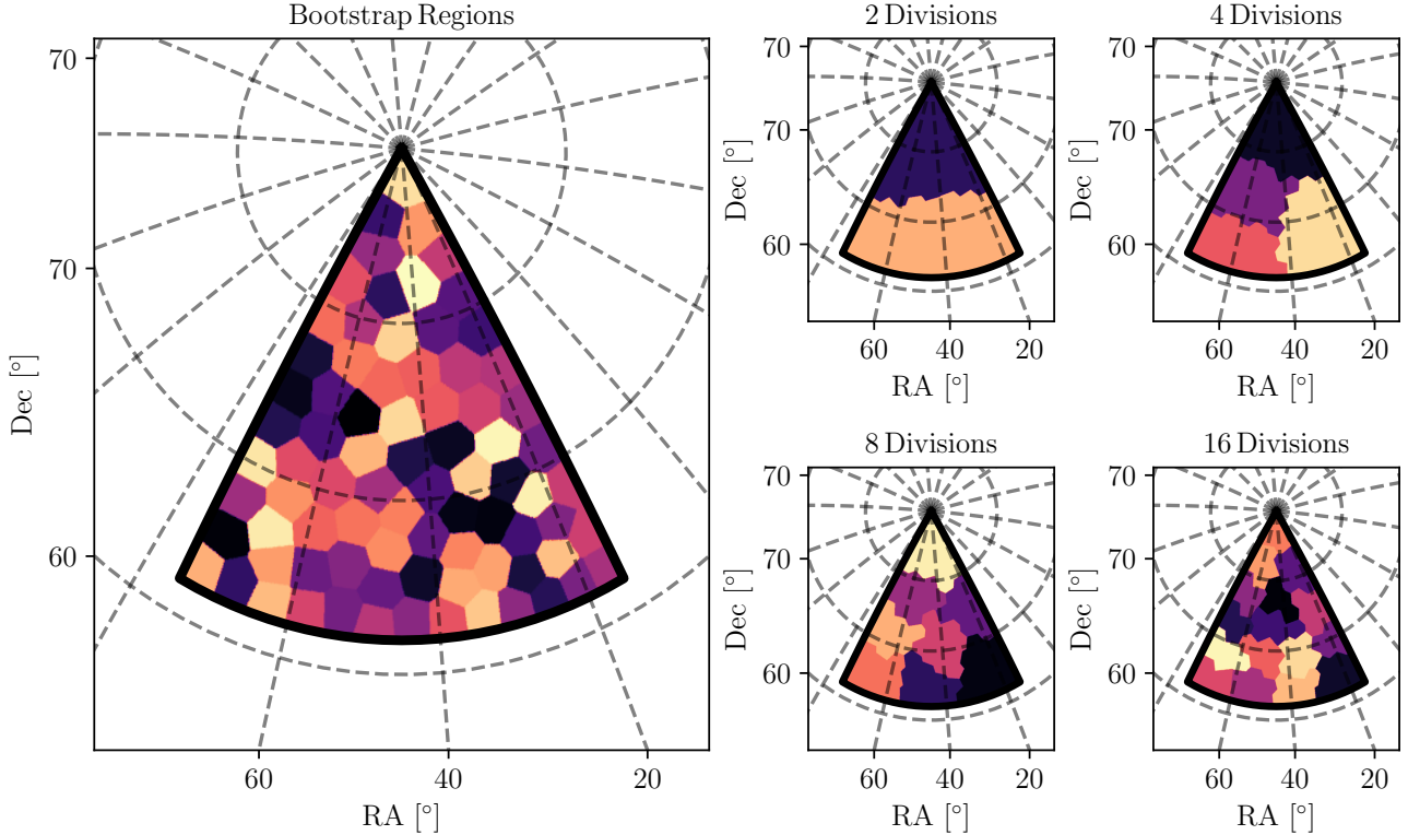
Fig. 4. Flagship footprint and area rescaling subregions. Left: bootstrap subregions, indicated with different colours, that are used to calculate errors in YAW. Right: different subregions of the Flagship footprint, shown with different colours, used to establish the relation between the tracer–target overlap area and the uncertainty on the mean redshifts of tomographic bins. The four subpanels show the Flagship footprint divided into 2 ( top left ), 4 ( top right ), 8 ( bottom left ), and 16 ( bottom right ) subregions. These are plotted on an orthographic projection of a subset of the sky focused on the Flagship footprint. The RA and Dec grid is shown with dashed grey lines. The values of the grid lines are indicated where they intercept the x -axis for the RA grid and the y -axis for the Dec grid.
