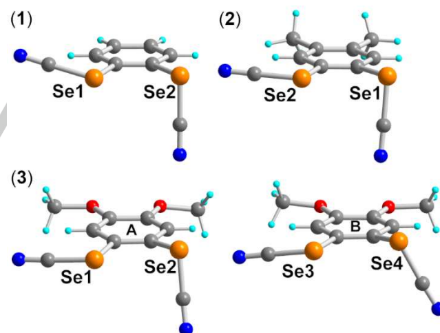
Figure 1. Details of the crystal structures of 1–3 . Note the two crystallographically independent molecules (A, B) in 3 . Intramolecular Se···Se distances amount to 3.245(1) Å in 1 , 3.237(1) Å in 2 , and 3.216(6) and 3.221(7) Å in 3A and 3B respectively.
