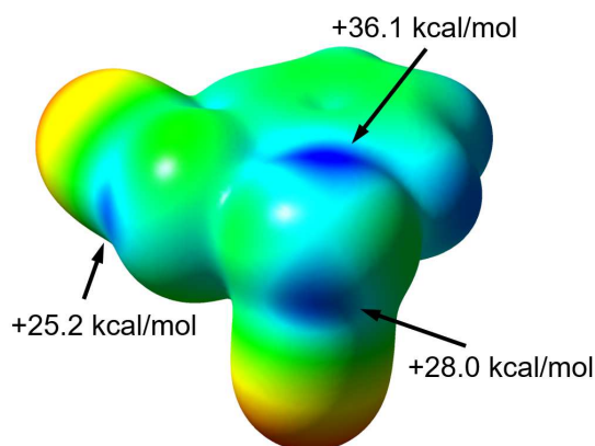
Figure 2. Electrostatic Potential (ESP) surface (plotted on the 0.002 e/\text{bohr}^3 isosurface of the electronic density) for compound 1 . Color range from -37.7 (red) to +43.9 (blue) kcal/mol.
