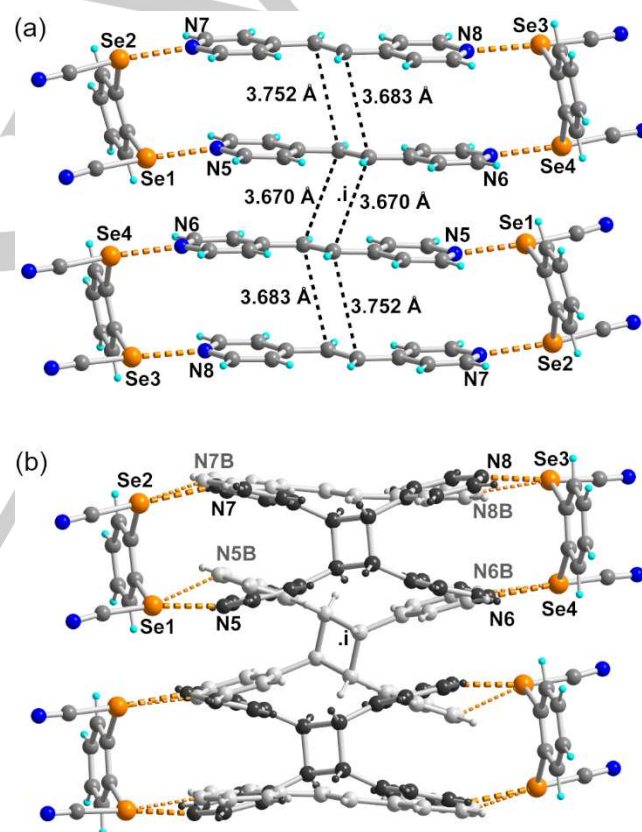
Figure 3. (a) Details of the solid-state association of rectangular, chalcogen bonded motifs in (\mathbf{1})_4(\mathbf{bpen})_5 . ChB are indicated by orange dotted lines, and short C\cdots C contact between ethylenic moieties by black dotted lines. (b) Details of the solid-state association after UV-irradiation and formation of the cyclobutane adducts. Occupation parameters for the two components (shown with atoms in black and light grey) are 0.661(6) and 0.339(6).
