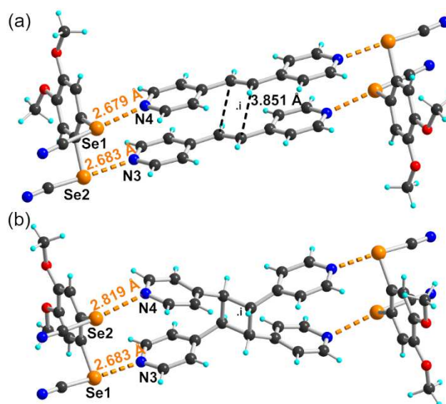
Figure 4. (a) Details of the solid-state association within a rectangular chalcogen-bonded motif in (3)( bpen ) 2 . ChB are indicated by orange dotted lines, and short C...C contact between ethylenic moieties by black dotted lines. (b) Details of the solid-state association of the same motif, after UV-irradiation and formation of the cyclobutane ring.
