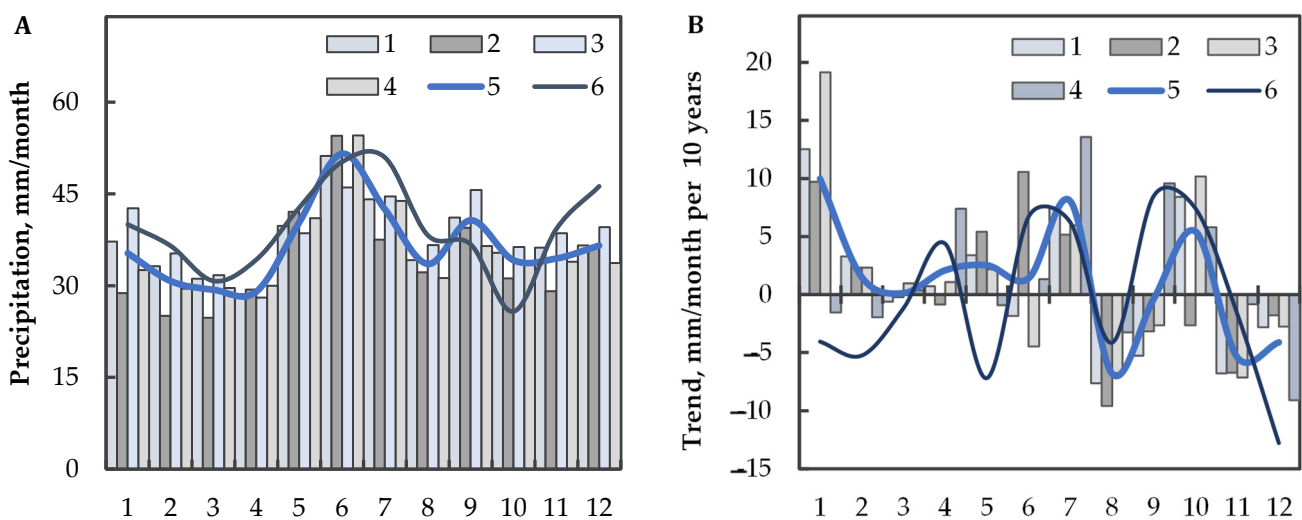
Figure 3. Seasonal variation of precipitation (A) and corresponding trends (B): monthly precipitation values for meteorostations Zaporizhzhia (1), Mikolaiv (2), Odesa (3), and Kherson (4) as well as for the whole region (5), for the period 1991–2020; 6—values of the climatic norm for the period 1961–1990.
