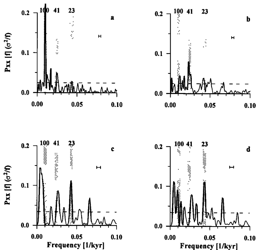
Figure 7. Results of harmonic analysis calculated on (a) TOC and (b) TOC MAR of ODP Site 723 [Emeis, 1993, Emeis et al. , 1995] and (c) TOC and (d) TOC MAR of core MD 900963 [Rostek et al. , 1994, 1997] using the software program SPECTRUM [Schulz and Stettgen, 1997]. A Fischer/Siegel test (dashed line) for compound periodicity was employed, and significant peaks outside the eccentricity (100), obliquity (41), and precession band (23) are labeled separately. Horizontal bar marks 6 dB bandwidth for each calculation.
