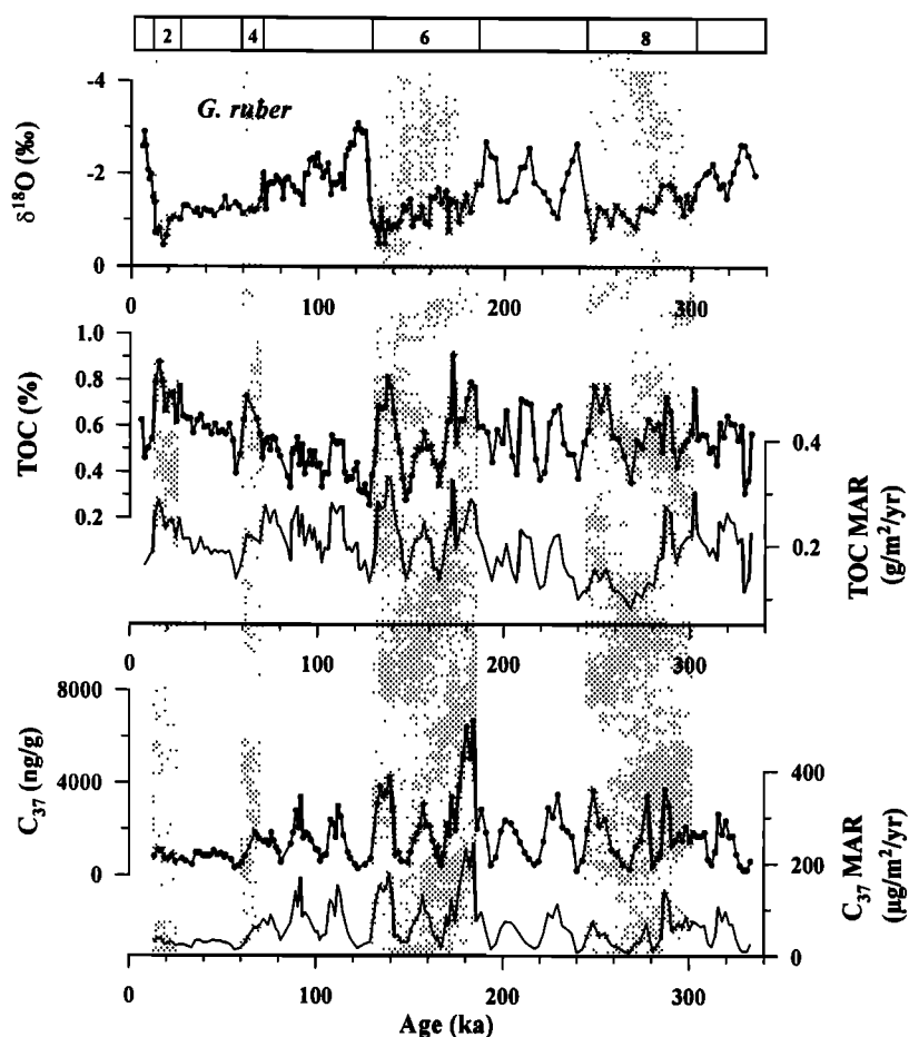
Figure 6. Time series of \delta^{18}\text{O} of the planktonic foraminifera Globigerinoides ruber , TOC, TOC MAR, C_{37} and C_{37} MAR for MD 900963 [Rostek et al., 1994, 1997].
