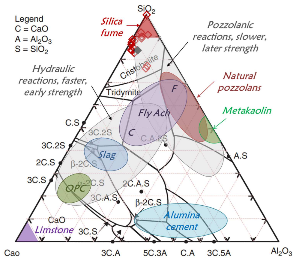
128 129 Fig. 1: Composition of TMS (black), composition of ground glass powder cf. [25–34], 130 superimposed on mainly used SCMs, adapted from [35,36]
