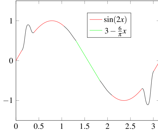
Figure 1: Example of a function \psi in [0, \pi]
