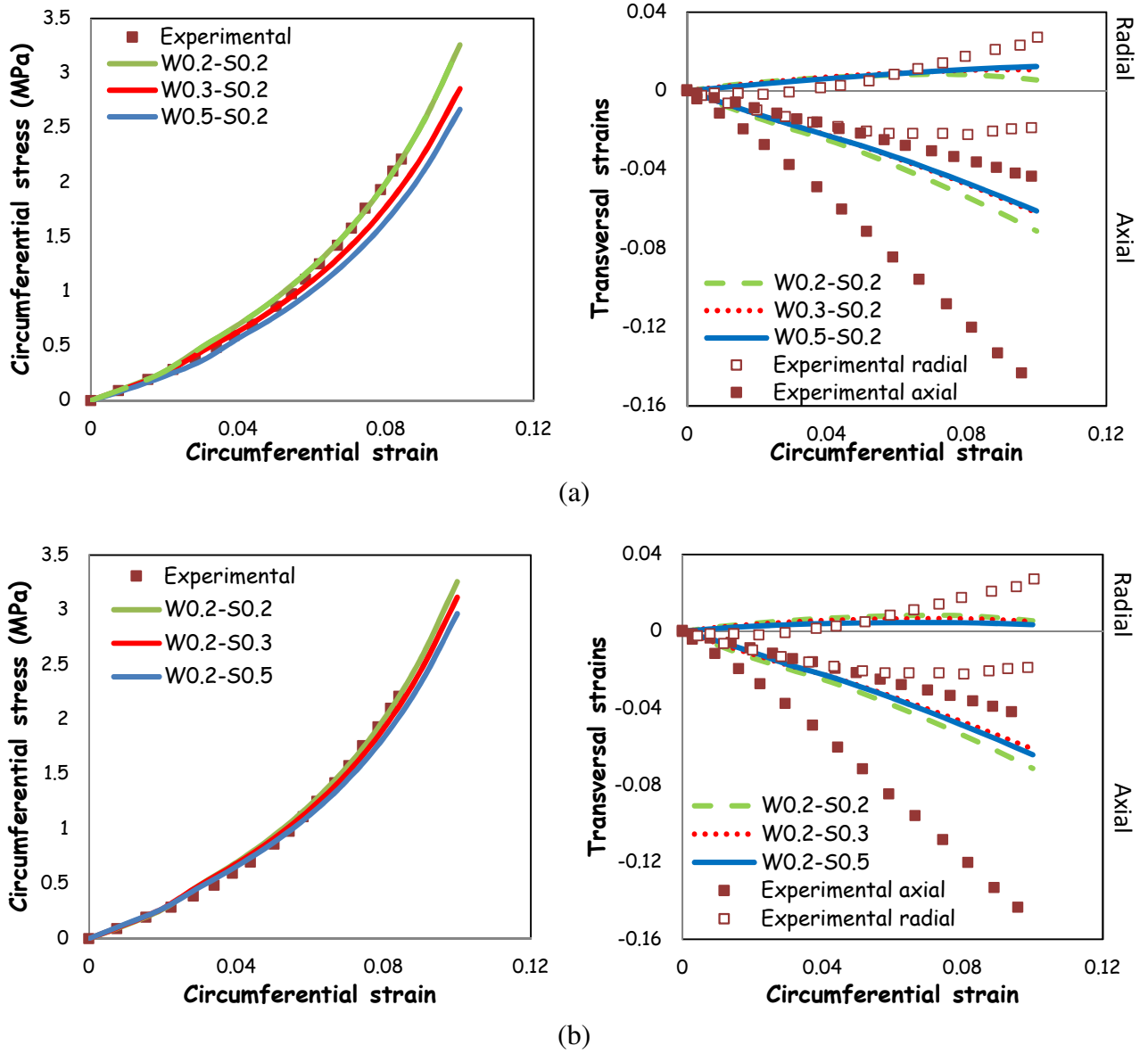
Figure 5. Mesostructure effects on nonlinear stiffness and transversal strain history in axial/radial directions: (a) cell walls thickness and (b) sheets thickness. The experimental stress-strain data are extracted from [17] and correspond to the anterior outer disc region; the experimental transversal strain data correspond to the extremum values reported in [19].
