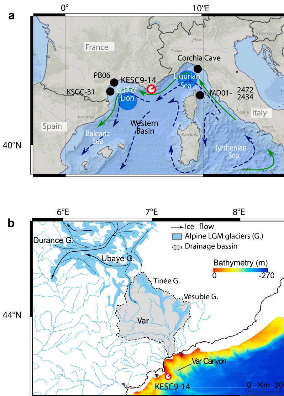
Fig. 1. Regional Map. a. Map of the Western Mediterranean basin showing the location of the main paleorecords discussed in the text: the lagoon core PB06 (43°30' N; 3°52' E, Sabatier et al., 2012) and the marine core KSGC-31 (43°0'23'' N; 3°17'56'' E, 60 m water depth; Jalali et al., 2016) from the Gulf of Lion, the marine cores MD01-2472 and MD01-2434 from Corsica Trough (respectively located at 42°36'42'' N; 9°43'97'' W; 501 m water depth and 42°22'51'' N; 9°47'04'' E; 780 m water depth, Toucanne et al., 2012) from the Ligurian Sea and the speleothem record from Corchia cave (43°59' N; 10°13' E, Zanchetta et al., 2007). The blue dashed arrows show the main path of the intermediate water mass (Levantine Intermediate Water) and the green arrows show the surface current/Northern Current (Millot and Taupier-Letage, 2005). The blue circles represent the convection areas where deep water masses are formed. b. Detailed map (adapted from Jorry et al., 2011) focused on the study area and showing the Var drainage basin as well as the bathymetric features of the sampled sediment core KESC9-14. (For interpretation of the references to colour in this figure legend, the reader is referred to the web version of this article.)
