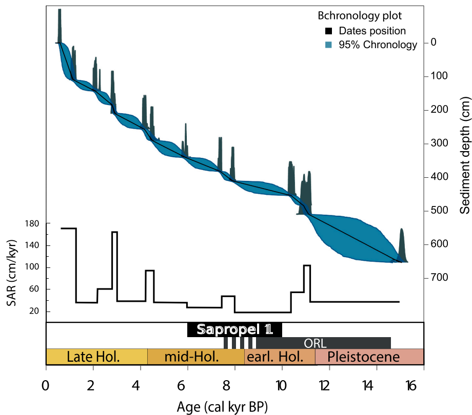
Fig. 2. Age model and sediment accumulation rate (SAR) of core KESC9-14. Age model was calculated using IntCal20 curve in Bchron R package (R Core Team, 2013). The Saproel 1 event was reported as defined by Hennekam et al. (2014) in the Eastern Mediterranean. The last ORL was defined in western Mediterranean from ~14.5 to 9–8 ka by Cacho et al., 2002 but can be regionally prolonged until 7 ka (Incarbona and Sprovieri, 2020).
