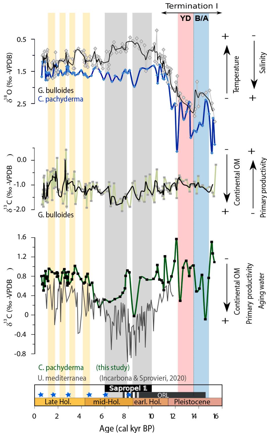
Fig. 4. Stable isotopic records from core KESC9-14. Age plots of benthic ( C. pachyderma ) and planktic ( G. bulloides ) \delta^{13}\text{C} and \delta^{18}\text{O} records from core KESC9-14 along with their environmental interpretations. Note that the values of \delta^{18}\text{O} are in inverse order to match the conventional Glacial-Interglacial marine isotopic reading. For G. bulloides \delta^{18}\text{O} and \delta^{13}\text{C} , the tick black curves represent the 3-point moving average. The main events and climate phases are reported similarly to Fig. 2.
