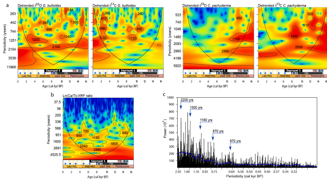
Fig. 10. Spectral analyses of main proxies used in core KESC9-14. a. Wavelets analyses of planktic and benthic stable isotopic data from core KESC9-14. b. Wavelets analyses of selected XRF proxies from core KESC9-14. The lines mark the 95% confidence level ( p = 0.05 ). c. Graphic representing the compilation of REDFIT analyses based on the relative abundance records of the 21 main benthic foraminifera species. The blue line marking the mean REDFIT spectrum. (For interpretation of the references to colour in this figure legend, the reader is referred to the web version of this article.)
