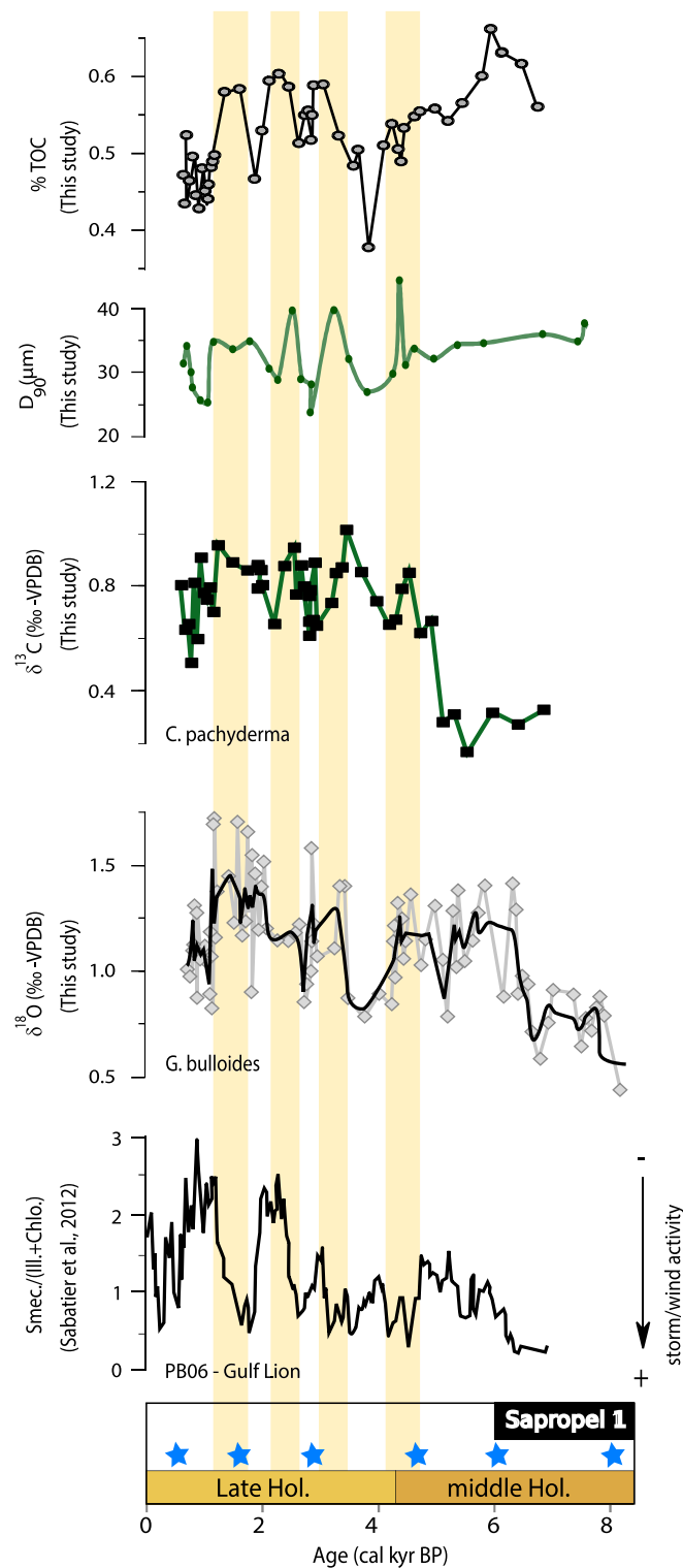
Fig. 9. Main features of the Holocene record from core KESC9-14 and comparison with nearby data. From bottom to top, we present a storm index obtained from the sediment composition of PB06 core (Sabatier et al., 2012) collected from a lagoon in the Gulf of Lion and the planktic \delta^{18}\text{O} , benthic \delta^{13}\text{C} , D90 and TOC content from our studied KESC9-14 core. The main events and climate phases are reported similarly to Fig. 2.
