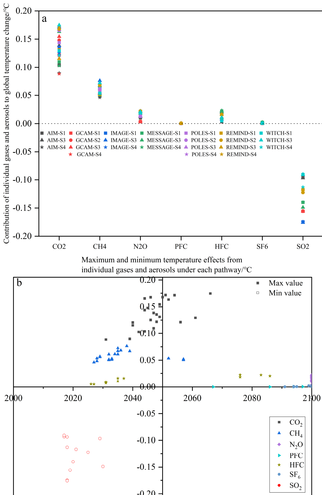
Figure 4. China's contribution to the global mean temperature from individual GHGs and air pollutants. (a) Maximum gas-by-gas contributions (in absolute terms) of China's emissions to the global mean
