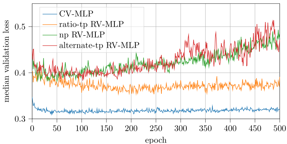
Figure 5 Real-Valued Equivalent-MLP comparison.
