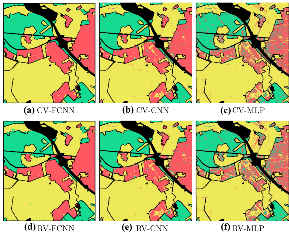
Figure 7 Comparison between model predictions. A Built-up Area; B Wood Land; C Open Area.
