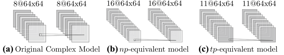
Figure 2 Real equivalent convolution example of a middle hidden layer. Figures generated using alexlenail .
