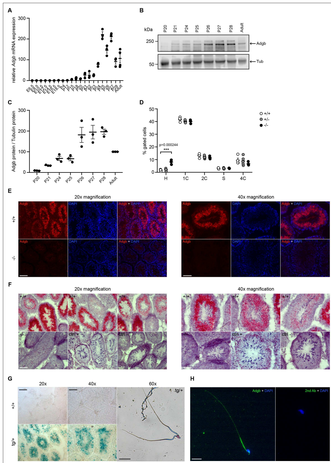
Figure 2. Testicular Adgb expression pattern and localization. (A) Relative mRNA expression levels of Adgb in testes of wild-type mice during embryonic development (E) and early post-natal (P) life (n=3–4 per condition). (B) Representative immunoblot for Adgb in testis lysates from wild-type mice at different P ages (n=3 per condition) and (C) corresponding protein quantification. Tubulin was used as loading control. (D) Flow cytometric analysis of spermatogenic cell populations following propidium iodide staining in Adgb wild-type (+/+, white circles, n=4), heterozygous (+/-, gray
