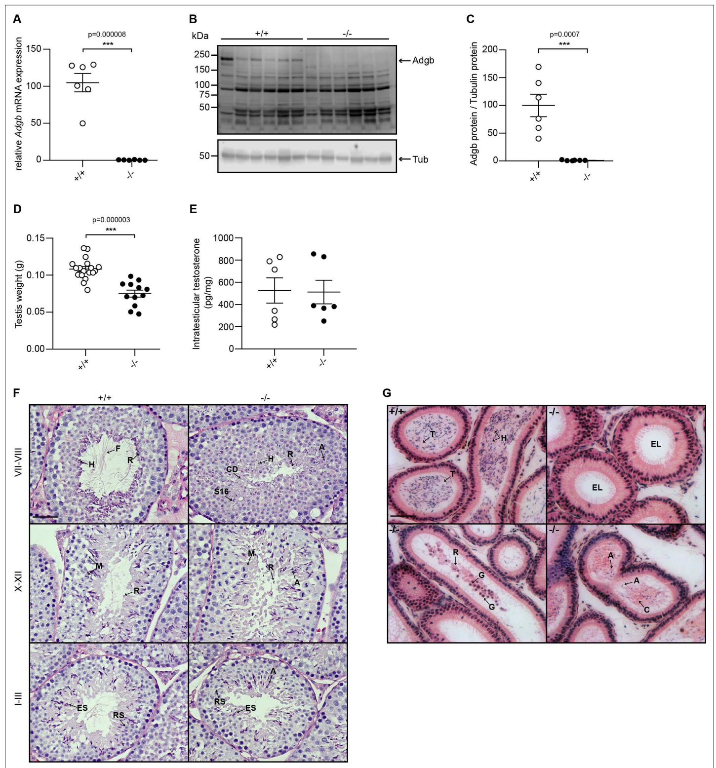
Figure 1. Validation of the knockout model and testicular phenotype. (A) Relative mRNA expression levels of Adgb in testes of wild-type (+/+) and knockout mice (-/-) ( n=6 per genotype; p=0.000008 ). (B) Representative immunoblot for Adgb in testis lysates from wild-type (+/+) and knockout mice (-/-) ( n=6 per genotype) and (C) corresponding protein quantification. Tubulin was used as loading control. p=0.0007 . (D) Testis weight (g) in Adgb wild-type (+/+), heterozygous (+/-), and knockout (-/-) mice ( n=8-13 per genotype). p=0.000003 . (E) Intratesticular testosterone levels (pg/mg) in Adgb wild-type (+/+) and knockout (-/-) mice ( n=6 per genotype). (F) Representative periodic acid Schiff (PAS)-hematoxylin-stained sections of testes from Adgb wild-type (+/+) and knockout mice (-/-) at the different stages of spermatogenesis. Heads (H), flagella (F), residual bodies (R), cytoplasmic debris
