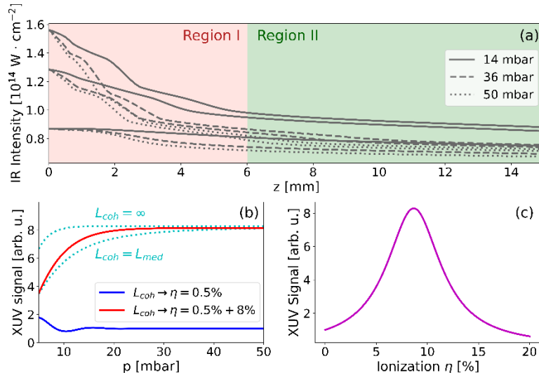
Fig. 1 (a) Results of numerical simulations of a 30 fs pulse propagating in krypton demonstrating the stabilization of the on-axis intensity in region II for different medium pressures and input laser intensities. In region I the intensity drops rapidly. (b) 17 th harmonic signal versus gas pressure obtained from the analytical model of Ref. [5], when the optimal signal is in the range L_{coh} > L_{med} (cyan dotted curves). The expected signal from region II shown in Fig. 1a) is denoted by the blue curve. By adding a constant pre-ionization of 8% to achieve phase-matching, the expected signal moves into desired region (red curve). (c) The absorption-limited XUV signal as function of ionization ratio \eta according to the same model of Ref. [5], which surprisingly does not depend on the medium density [6].
