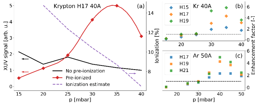
Fig. 2 (a) Experimentally measured intensity of the 17th harmonic order as a function of pressure for HHG in Kr without pre-ionization (black curve) and in pre-ionized medium with discharge peak currents of 40 A (red diamonds) [6]. Red line (spline) is added to guide the eye. Estimate of degree of ionization in the (purple dashed curve). (b) Enhancement factor for H15 (blue), H17 (orange), and H19 (green diamonds) in krypton with 40 A peak current. (c) Enhancement factor for H17 (blue), H19 (orange), and H21 (green squares) in argon with 50 A peak current. Each experimental point corresponds to the strongest shot from a set of ten laser shots.
