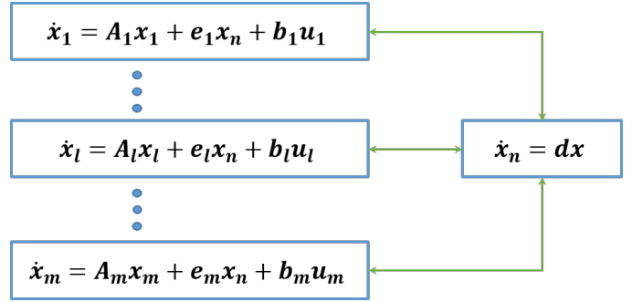
Fig. 1. Network of interconnected linear control systems with star topology.
