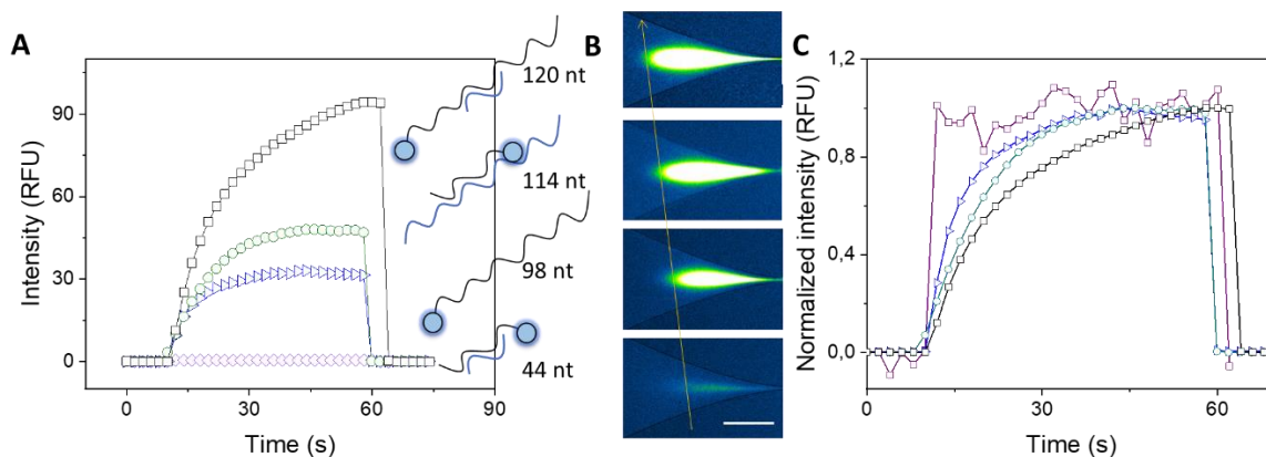
Figure 3. Optimization of target and probe size for biosensing. (A) The plot shows the concentration kinetics for a series of targets of increasing size of 44, 98, 114, and 120 nt (pink, blue, green and black dataset, respectively). v_0^{max} is set to 30 mm/s and E^{max} is 23 kV/cm. (B) The fluorescence micrographs correspond to the signal recorded after 50 s of actuation for the 44, 98, 114, and 120 nt targets from bottom to top. The scale bar corresponds to 200 \mu m. (C) The graph reports the same curves as in (A) after normalization in intensity.
