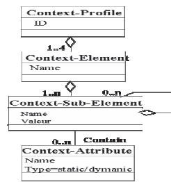
Fig.7. General structure of our context model
