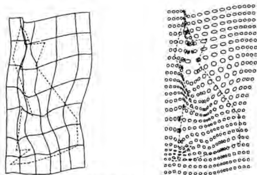
FIG. 7. Gough Map. Left: Warped Grid of Latitude and Longitude; The Transformed Image. Right: Tissot's Indicatix, Image, Strain Tensor
