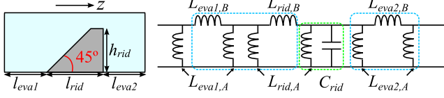
Fig. 2. Chamfered ridge: longitudinal cut and circuit model.
