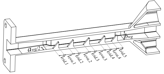
Fig. 6. Inner view of the manufactured EMF. Dimensions (in mm): a_{wg} = 13.0 , b_{wg} = 8.0 , w_{rid} = 3.0 , h_{rid,i} = \{5.3, 5.4, 5.3, 5.3, 4.6\} , l_{rid,i} = \{5.6, 5.8, 6.1, 6.1, 5.9\} , and l_{eva,j} = \{9.3, 10.6, 9.9, 6.9\} .
