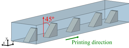
Fig. 1. Example of the proposed vertically printable EMF.
