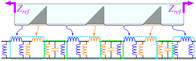
Fig. 4. Longitudinal section of a N = 3 filter with the chamfered ridge and its corresponding equivalent circuit.
