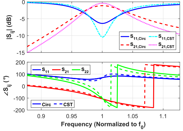
Fig. 3. FW [computer simulation technology (CST)] and circuitual simulation of an evanescent WG loaded with a chamfered ridge resonator.
