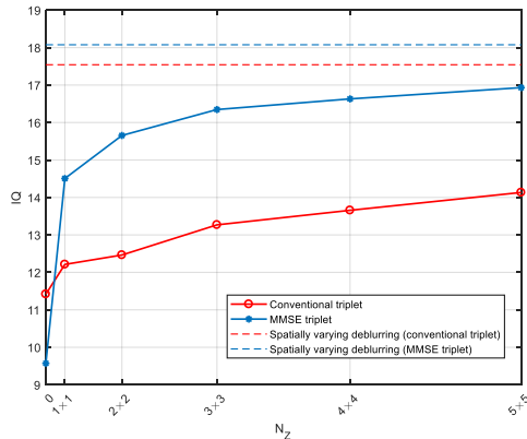
Figure 11: IQ on the simulated image (Barbara) as a function of the number of areas for piecewise Wiener deconvolution, for the conventional triplet and the MMSE triplet. N_Z = 0 means that there is no deconvolution. The performance in case of spatially varying deblurring is indicated by a dotted line.
