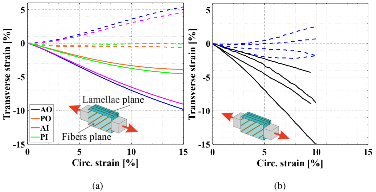
Figure 6. Multi-lamellae transverse responses under UA circumferential stretching for the different disc regions (solid lines: fibers plane, dashed lines: lamellae plane): (a) model results, (b) experimental data of Baldit [50].
