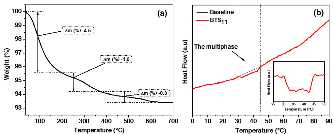
166 Fig.4 (a) ATG curve and (b) DSC heat flow curve of the BTS_{11} powder synthesized by the second approach at 180°C (The inset 167 shows the zoom region from 25 to 50 °C).
