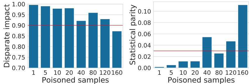
Figure 5: Verifying poisoning attack against fairness using FVGM. The red line denotes the safety margin of the ML model against the attack.
