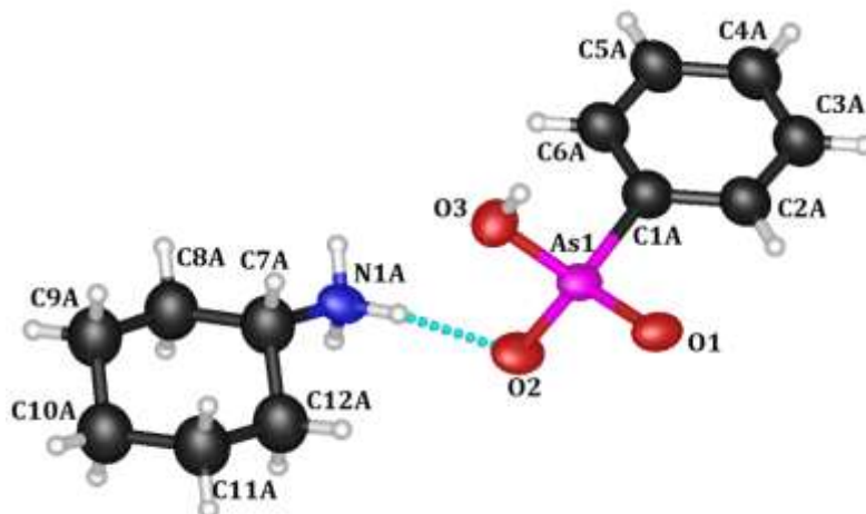
Fig. 5:- Molecular view of 2 showing 50% probability ellipsoids for atoms and the crystallographic numbering scheme adopted [atom color code: C, black; H, white; O, red; N, blue; As, pink]. Only one fragment of the disordered species is shown. Selected bond lengths and angles (Å, deg): O1–As1 1.662 (2), O2–As1 1.649 (2), O3–As1 1.719 (2), As1–C1A 1.927 (5), As1–C1B 1.890 (5), N1A–C7A 1.477 (7), N1B–C7B 1.477 (7); O1–As1–O2 115.53 (11), O1–As1–O3 111.13 (11), O1–As1–C1A 107.3 (2), O1–As1–C1B 108.5 (2), O2–As1–O3 103.84 (11), O2–As1–O1 104.03 (11), O2–As1–C1A 110.6 (2), O2–As1–C1B 110.2 (2), O3–As1–C1A 108.3 (2), O3–As1–C1B 107.3 (2), N1A–C7A–C8A 109.3 (6), N1A–C7A–C12A 109.3 (6), N1B–C7B–C8B 117.1 (19), N1B–C7B–C12B 115.8 (19).
