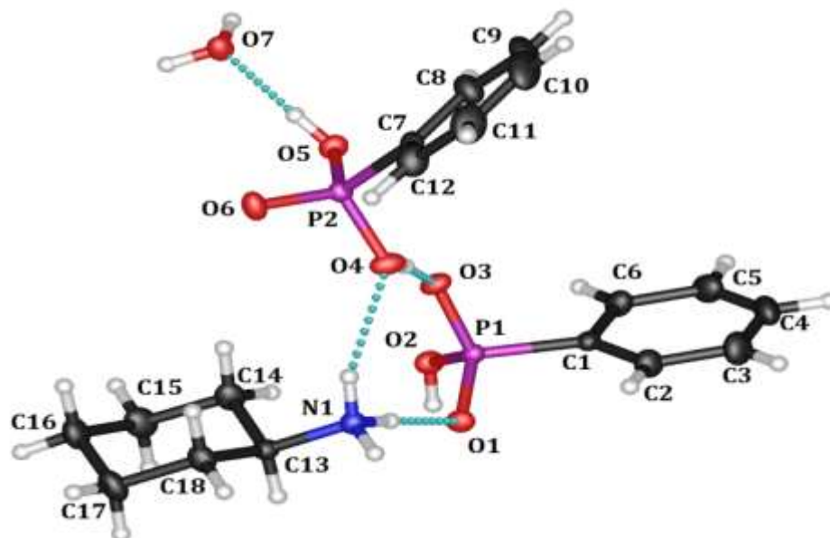
Fig. 1:- Molecular view of 1 showing 50% probability ellipsoids for atoms and the crystallographic numbering scheme [atom color code: C, black; H, white; O, red; N, blue; P, pink]. Selected bond lengths and angles (Å, deg): P1–O1 1.5097 (9), P1–O2 1.5646 (10), P1–O3 1.5152 (9), P1–C1 1.7959 (13), P2–O4 1.5509 (10), P2–O5 1.5511 (10), P2–O6 1.4915 (10), P2–C7 1.7912 (13), C13–N1 1.4987 (16); O1–P1–O2 112.42 (5), O1–P1–O3 115.21 (5), O3–P1–O2 105.20 (5), O1–P1–C1 108.64 (6), O2–P1–C1 106.95 (6), O3–P1–C1 105.20 (5), O5–P2–O4 105.84 (5), O6–P2–O5 114.05 (5), O6–P2–O4 111.38 (6), O4–P2–C7 106.95 (6), O5–P2–C7 108.06 (6), O6–P2–C7 110.21 (6), N1–C13–C18 110.25 (10), N1–C13–C14 109.72 (10).
