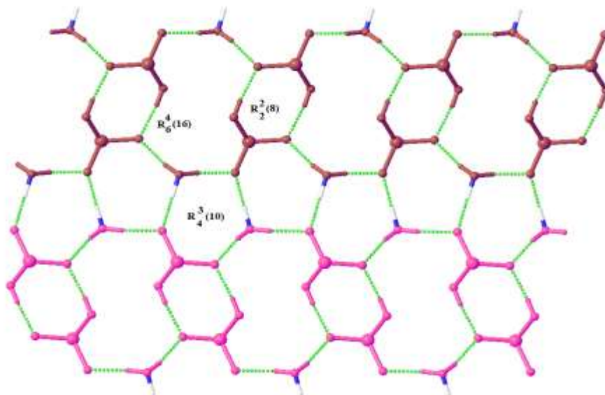
Fig. 6:- Molecular view of 2 showing 50% probability ellipsoids for atoms, showing the propagation of the infinite chain network. Phenyl and cyclohexyl groups are omitted for clarity.
