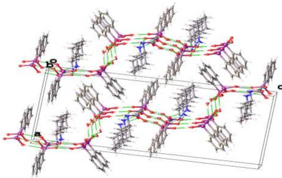
Fig. 4:- Molecular partial packing diagram of 1 showing 50% probability ellipsoids for atoms, showing the pleated layer network.
