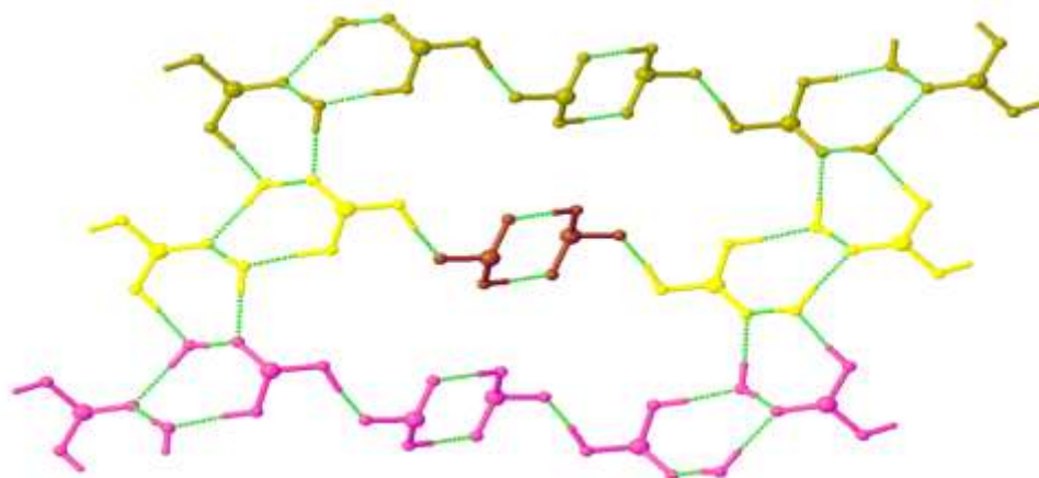
Fig. 2:- Molecular view of 1 showing 50% probability ellipsoids for atoms, showing the two different dimers and chains connected into an anionic layer network. Phenyl groups are omitted for clarity.
