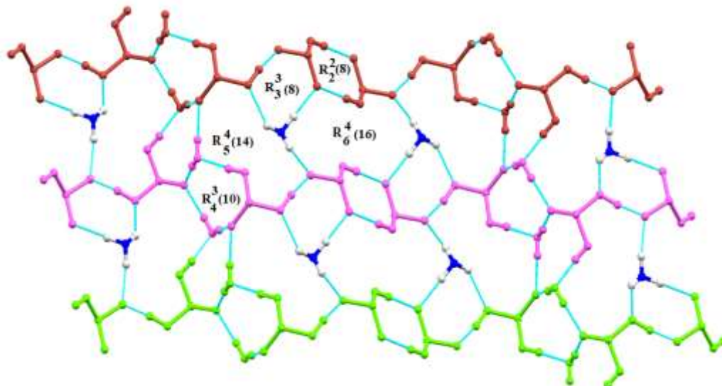
Fig. 3:- Molecular view of 1 showing 50% probability ellipsoids for atoms, showing the interactions of cations slipped in between the chains growing the layer network. Phenyl and cyclohexyl groups are omitted for clarity.
