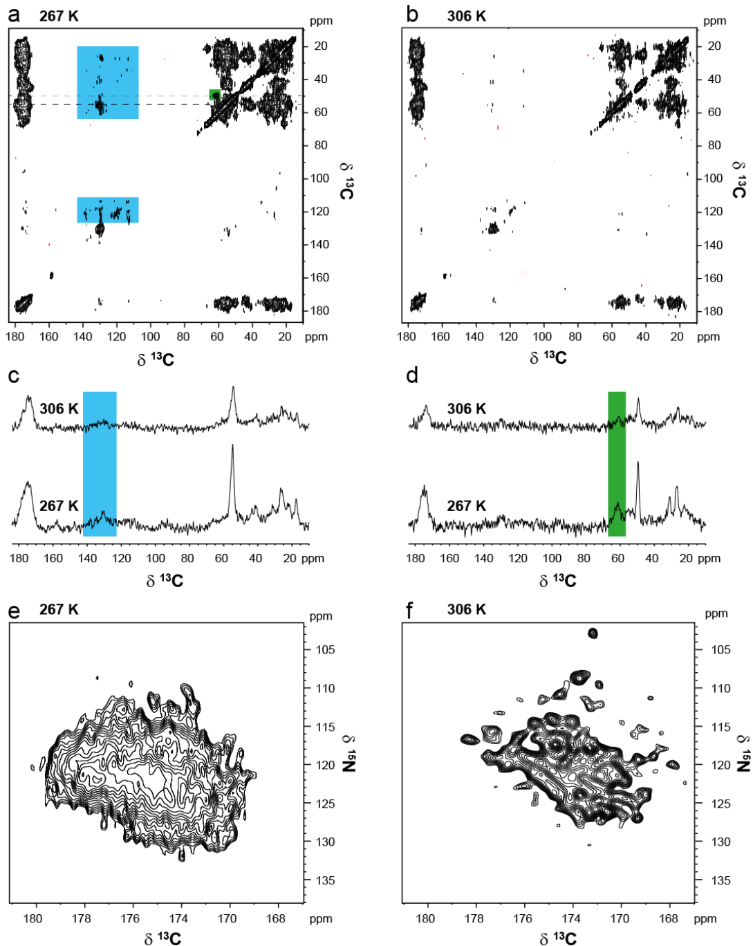
Figure 3: 2D ^{13}C - ^{13}C DARR spectra recorded at 10 kHz MAS with 100 ms mixing (a, b) and ^{15}N - ^{13}CO (e, f) of mTSPO at two temperatures (267 and 306 K). Regions with increased polarization transfer at 267 K are highlighted in blue and green on the DARR spectrum. Two rows (c, d) extracted from the DARR spectra at 267 and 306 K illustrate the improved transfer at 267 K. The following experimental parameters were used in the different spectra: 128 transients, 2s repetition delay for the DARR spectra (a, b); 512 transients, 2s repetition delay for the NCO spectra. The following apodisation functions have been used: cosine square function in the indirect dimension and exponential decay corresponding to 20 Hz line broadening factor for DARR and exponential decay corresponding to 20 Hz line broadening factor in both dimensions for the NCO spectra, respectively.
