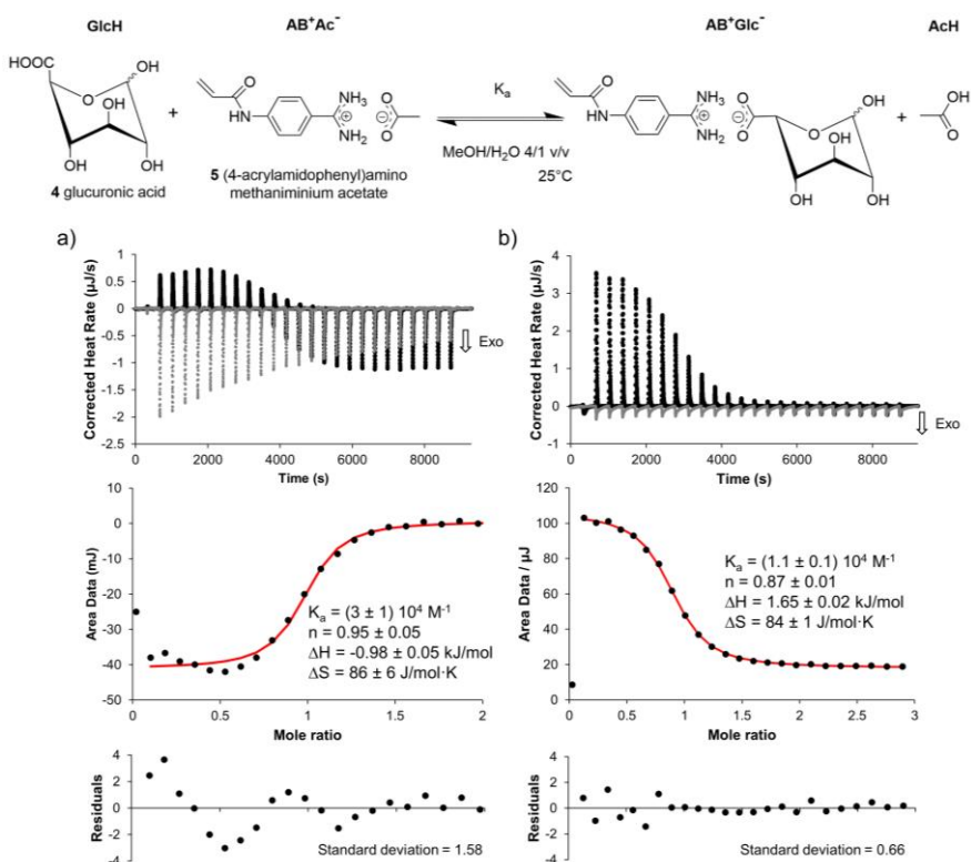
Figure 4: Direct (a) and reverse (b) titrations of AB + Ac - (5) into GlcH (4) in MeOH/H 2 O (4/1 v/v) at 25°C as filled black circles. The dilutions of 4 and 5, respectively, into MeOH/H 2 O (4/1 v/v) are also shown as grey filled circles. The middle thermogram shows the integrated heat data as filled black circles and the nonlinear fitting of the data using the 1:1 independent binding model as red continuous line.
