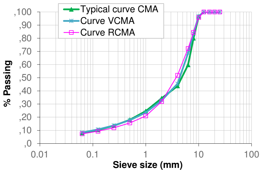
Fig. 2 Grading curves for virgin and recycled asphalt mixtures.
