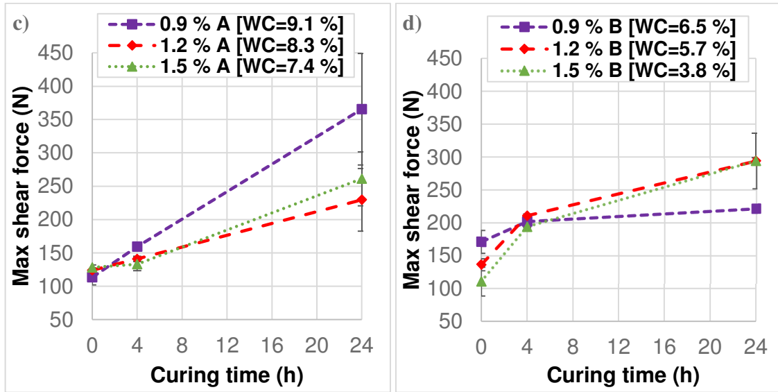
Fig. 8 Cohesion build-up kinetics of VCMA produced with surfactant A (a) and surfactant B (b) and RCMA manufactured with surfactant A (c) and surfactant B (d). Curing conditions: 35 °C, 20 % relative humidity.
