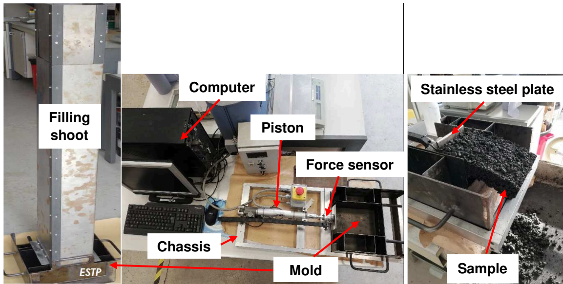
Fig. 3 Spreadability-meter device.
