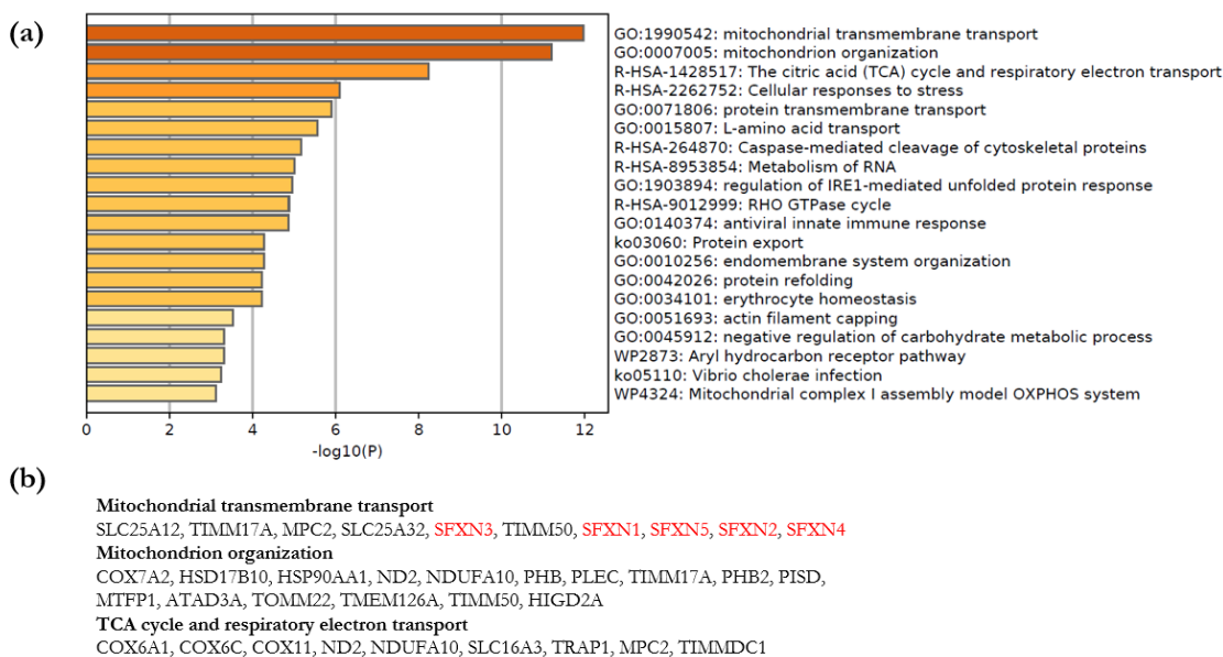
Figure 4. Metascape Enrichment analysis for SFXN1 partners. (a) Metascape bar graph for viewing top non-redundant enrichment clusters, one per cluster, using a discrete color scale to represent statistical significance (dark orange for the most significant clusters). (b) Hits from the top 3 enrichment clusters (mitochondrial transmembrane transport, mitochondrion organization, TCA cycle and respiratory chain).
