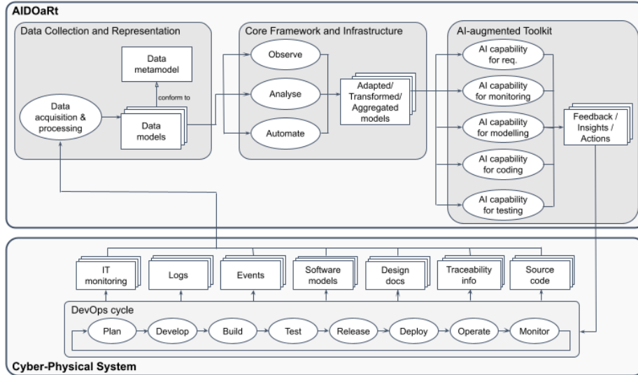
Figure 3: AIDOaRt Approach
