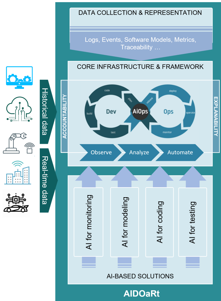
Figure 2: AIDOaRt Conceptual Architecture
