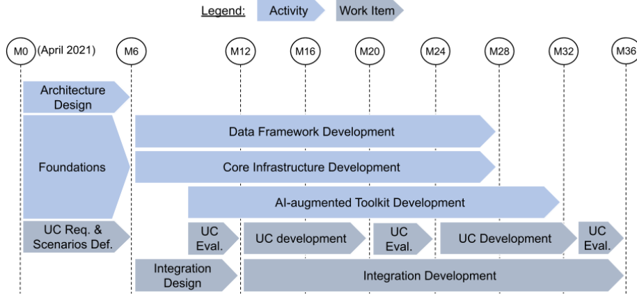
Figure 5: AIDOaRt Timeline
