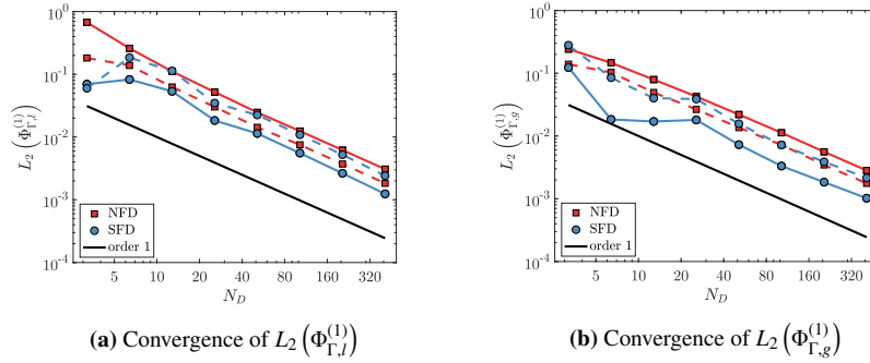
Figure 9: Mesh convergence of L_2(\Phi_{\Gamma,i}^{(1)}) and L_2(\Phi_{\Gamma,g}^{(1)}) for normal finite differences (NFD) and dimensional-splitting finite differences (SFD) using first-order (—) or second-order discretization (---).
