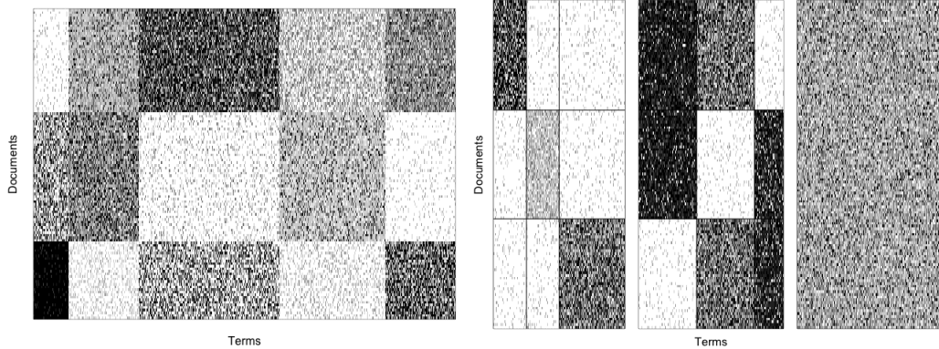
Figure 17: Left : the usual Poisson Latent Block Model: we see that some blocks are not easily classifiable into noisy or significant blocks. Right : the SOCC alternative approach: we easily distinguish the noisy blocks (lighter ones) and the significant ones (darker ones).
