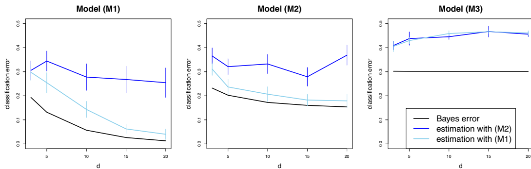
Figure 14: Classification error as a function of the dimension d , when n = 30 observations are generated from model (M_1) on the left, (M_2) on the center and n = 100 observations from model (M_3) on the right. In each case, the theoretical Bayes error is drawn in black, the estimation error with (M_1) in cyan and with (M_2) in blue. Errors are averaged on 50 replications and vertical bars represent 95% confidence intervals.
