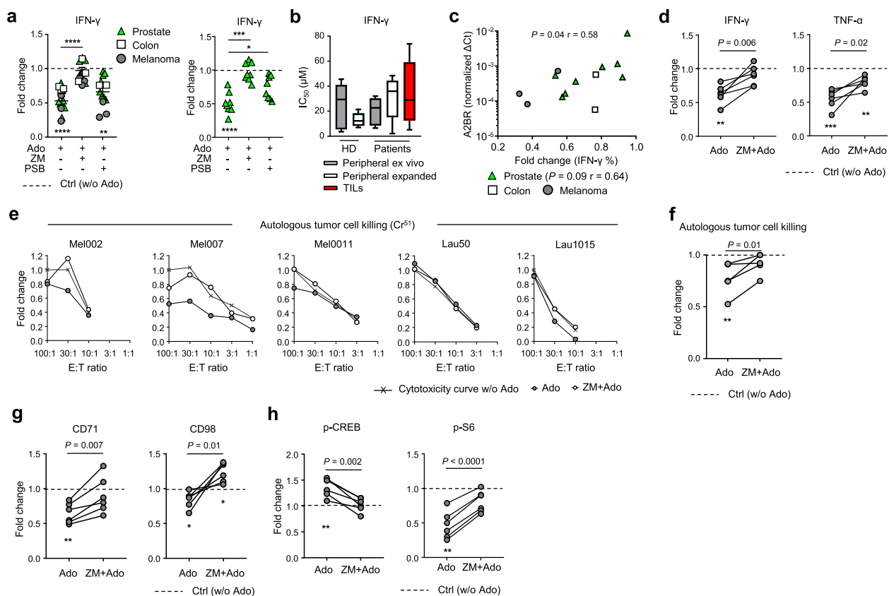
Fig. 4 Ado impairs TIL effector functions and autologous tumor cell recognition. a Cumulative data of the fold change in CD8 + TIL IFN- \gamma production in the presence of the indicated combinations of Ado, A2AR agonist (CGS 21680) and A2AR/A2BR antagonists (ZM 241385 and PSB 1115, respectively) ( n = 14 ). The left graph shows all the TIL samples analyzed, while the right graph only shows prostate-derived samples. b Cumulative data of the functional sensitivity ( IC_{50} of IFN- \gamma production) to Ado measured in resting or expanded peripheral CD8 + T cells ( n = 5 ) derived from HD or patients and in CD8 + TILs ( n = 10 ) derived from patient tissues. The functional sensitivity was measured after overnight stimulation by anti-CD3/CD28-coated beads in the presence of decreasing concentrations of Ado. c Correlation between A2BR expression measured by qRT-PCR and the Ado-mediated fold change in IFN- \gamma production in CD8 + TILs. Spearman's test, n = 13 ( n = 8 for the prostate sample analysis). d Cumulative data of the fold change in IFN- \gamma and TNF- \alpha production by TILs stimulated overnight by autologous tumor cells in the presence of Ado or ZM 241385 + Ado. ( n = 6 ) e Each graph represents cytotoxicity curves for one patient quantified in the absence of Ado, in the presence of Ado or ZM 241385 + Ado. Data are presented as normalized to the cytotoxicity measured in the absence of Ado at the effector:target (E:T) ratio of 100:1. Cytotoxicity was measured by coincubating TILs for 4 h with autologous tumor cells; measurements were performed in triplicate. f Cumulative data of the fold change in cytotoxicity in the presence of Ado or ZM 241385 + Ado ( n = 5 ). g Cumulative data of the fold change in CD71 and CD98 expression by TILs stimulated overnight by autologous tumor cells in the presence of Ado or ZM 241385 + Ado ( n = 6 ). h Cumulative data of the fold change in p-CREB and p-S6 expression by TILs stimulated for 3 h by autologous tumor cells in the presence of Ado or ZM 241385 + Ado ( n = 6 ). In all charts, each dot represents a patient, and the mean and standard error are presented. In all box charts, the 25th to 75th percentiles, the median and min-max of the values are presented; * P < 0.05 , ** P < 0.01 , *** P < 0.001 . Paired t test and/or one-way ANOVA tests
