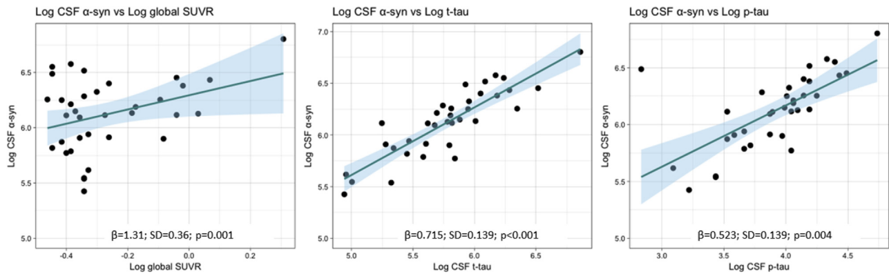
Fig. 1. Plots showing the association between CSF \alpha -synuclein and global SUVR, CSF \alpha -synuclein and CSF t-tau, and CSF \alpha -synuclein and CSF p-tau 181 : the univariate analysis. Notes. For each curve, \beta slope and standard deviation (SD) are indicated with respective P value (significant level P < .05 ) adjusted for age and sex. Abbreviations: CSF, cerebrospinal fluid; p-tau, hyperphosphorylated tau at Threonine site 181; t-tau, total tau; SUVR, standard uptake value ratios; Log, logarithmic transformation.
