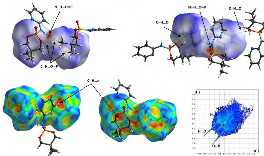
Figure 5. Views of the d_{\text{norm}} Hirshfeld (up) and shape index (down) surface maps plotted on the compound 2 in two orientations, introducing close contacts, along with the full fingerprint plot labeling features related to the main intermolecular contacts (down).
