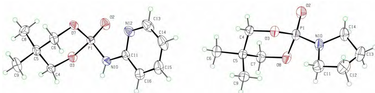
Figure 2. Views of Ellipsoid-style and atom-labelling presentation of molecular structures of 2 (left) and 3 (right) in the asymmetric unit. The 30% probability level has been allocated for drawing displacement ellipsoids and H atoms are drawn as circles of arbitrary radii.
