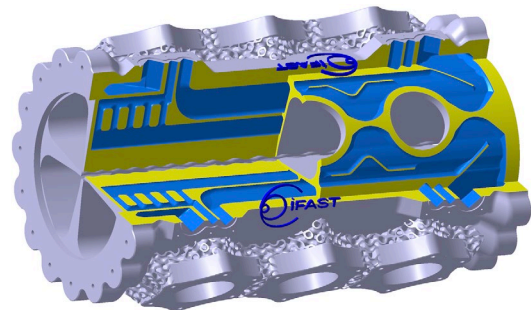
Figure 1: Full-size optimised RFQ.
