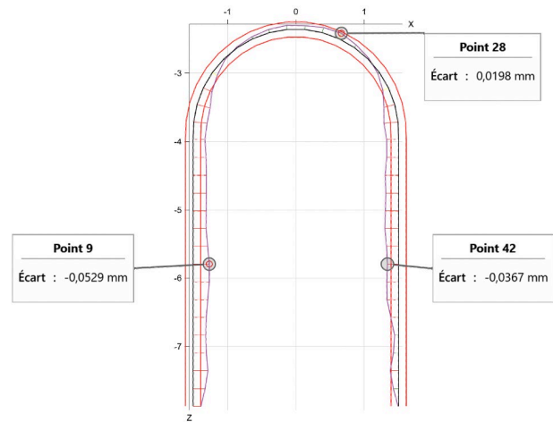
Figure 4: vane-tip and side measurements of 1/4 RFQ sample No1 – prior post-processing.
