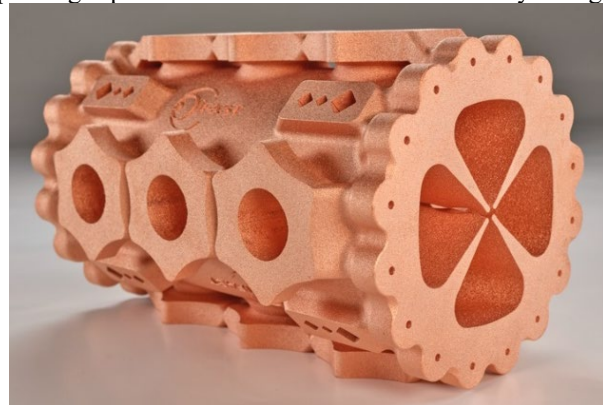
Figure 8: Full-size AM produced RFQ of pure copper.
