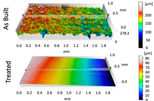
Figure 7: 3D surface roughness of the post-processed ¼ RFQ sample.
