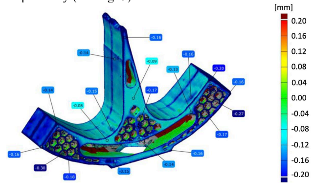
Figure 5: Measurements of 1/4 RFQ segment sample No1 - post-processed.
