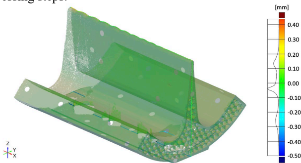
Figure 3: Deviation measurements of 1/4 RFQ sample No1 – prior post-processing.
