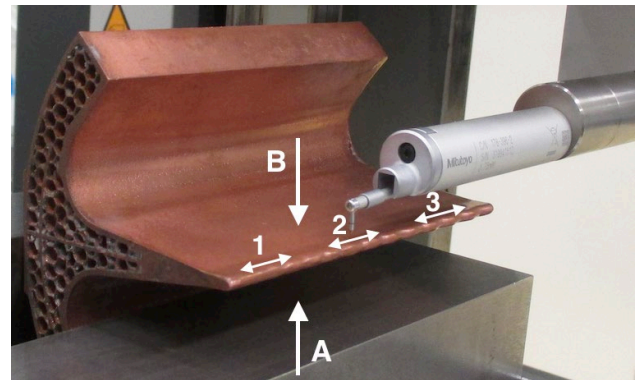
Figure 6: Measurements of 1/4 RFQ segment sample No2 - post-processed with MMP TECHNOLOGY®.
