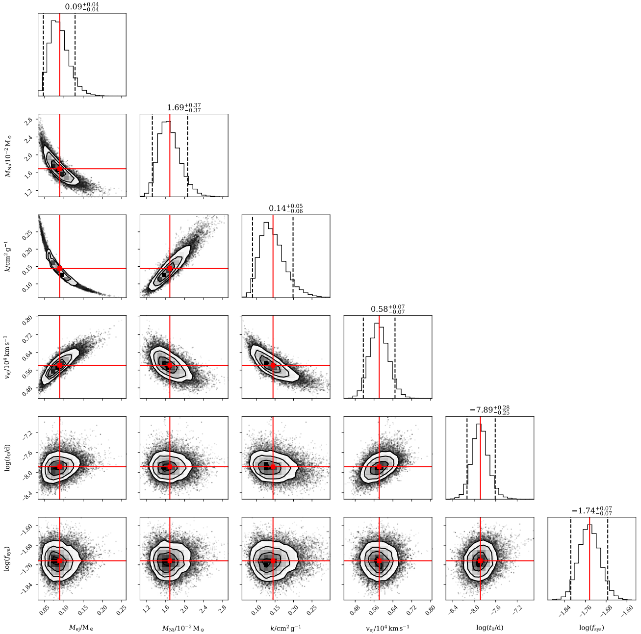
Fig. C.1. Corner plot showing marginalised one-dimensional and 2-dimensional posterior probability densities on the SN model parameters obtained by fitting the SN 2019wxt photometric dataset. The red lines and square markers show the estimated position of the maximum a posteriori . Dashed lines in the plots on the diagonal bracket 90% credible ranges. Contours in the two-dimensional plots show credible regions at the 68%, 95% and 99.7% credible level, while black dots are random samples from the posterior, qualitatively showing the behaviour outside the contours. The physical meaning of the parameters is described in the text.
