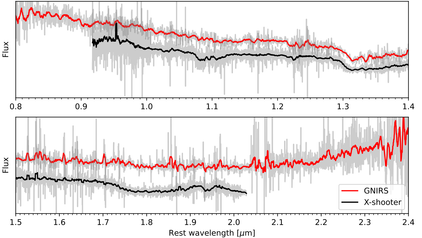
Fig. 5. NIR spectra for SN 2019wxt taken on 19 Dec 2019. Grey lines show original spectra, colour lines have been smoothed with a Savitzky-Golay filter with window length 50 \text{ \AA} . We do not include the GTC/EMIR spectrum which has low S/N.
