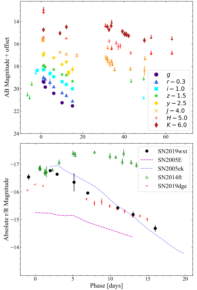
Fig. 2. Light curves. Top panel: grizyJHK light curves of SN 2019wxt. Lower panel: Comparison of absolute r and R -band light curves with those of other faint and rapidly evolving transients. For both panels, the phase is given with respect to the epoch of i -band maximum, i.e. MJD 58835.1.
