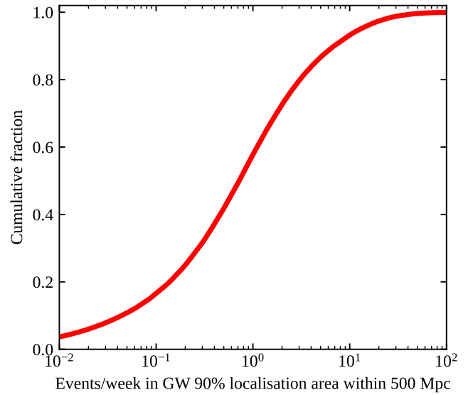
Fig. 16. Cumulative distribution of the expected number of SN2019wxt-like events per week within 500 Mpc that will happen within the 90% sky localisation region of GW candidates in O4.
