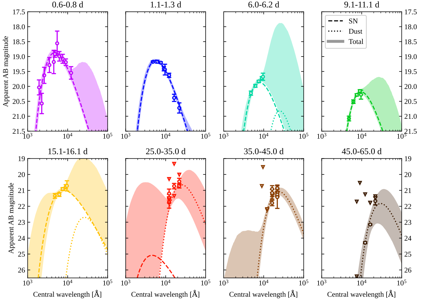
Fig. D.1. Spectral energy distributions fitted with a blackbody + dust model. Each panel shows a SED of SN2019wxt constructed by considering photometric measurements within a time window (annotated above each panel, in days post i -band maximum). The formally best-fitting blackbody (‘SN’) and modified blackbody (‘Dust’) components are shown by dashed and dotted lines respectively, while the filled regions span the 5th to the 95th percentile of the model (SN+Dust) magnitudes corresponding to the posterior samples at each wavelength. The fits are performed adopting log-uniform priors on the SN luminosity in the 10^{35} - 10^{43} \text{ erg/s} range and on the dust mass in the 10^{-6} - 10^{-3} M_{\odot} range, and uniform priors on the SN temperature in the 4000 – 20000 K range and on the dust temperature in the 100 – 2500 K range.
