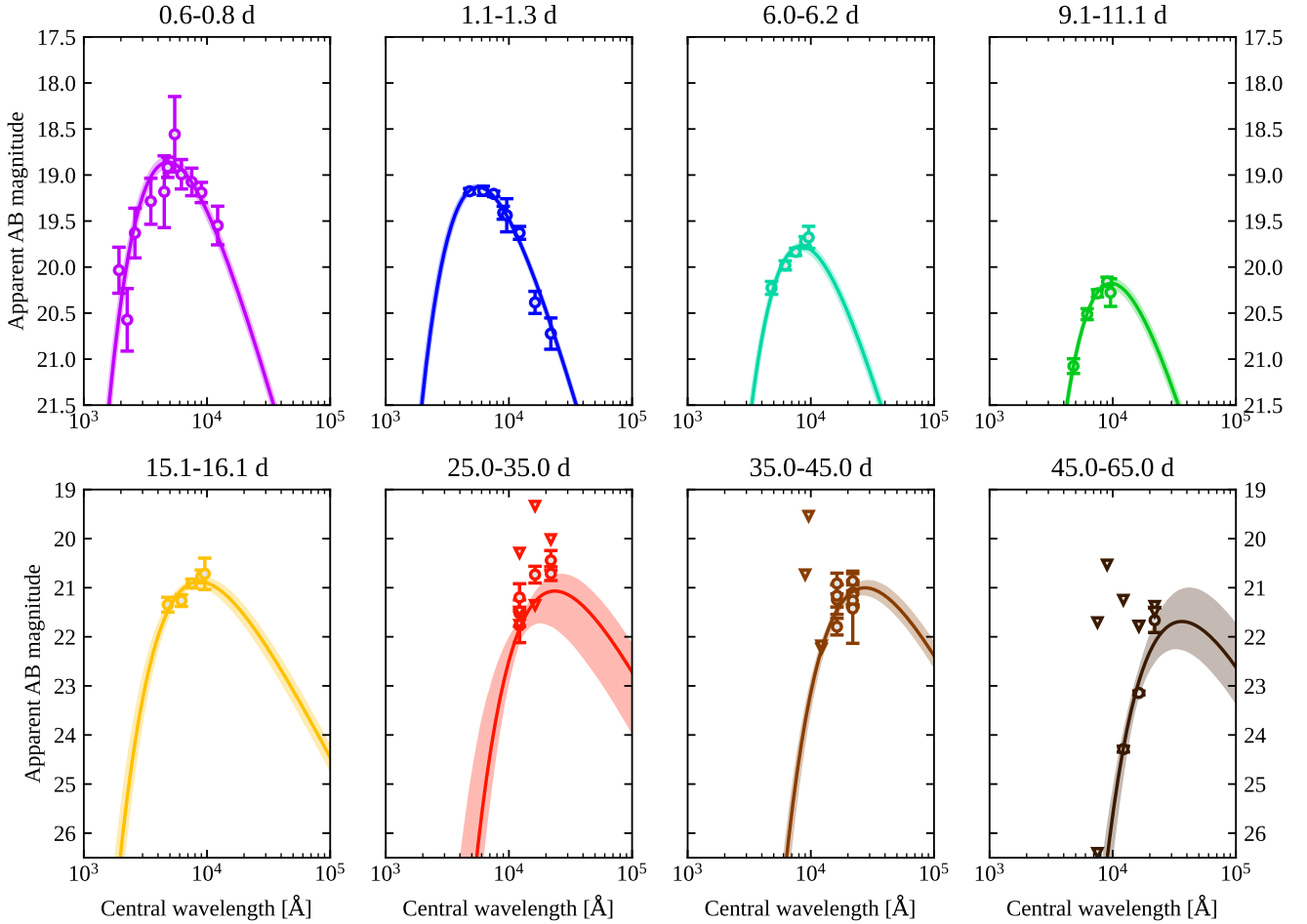
Fig. 7. Spectral energy distributions fitted with a blackbody model. Each panel shows a SED of SN2019wxt (circles represent detections with one-sigma error bars; triangles represent upper limits) constructed by considering photometric measurements binned within a time window (annotated above each panel, in days post i -band maximum). The formally best-fitting blackbody is shown by a solid line, while the filled regions span the 16th to the 84th percentile (equivalent to one-sigma uncertainties) of the model magnitudes corresponding to the posterior samples at each wavelength. The fits are performed adopting a log-uniform prior on the BB luminosity in the 10^{35} – 10^{43} erg/s range and a uniform prior on the temperature in the 1000–20 000 K range.
