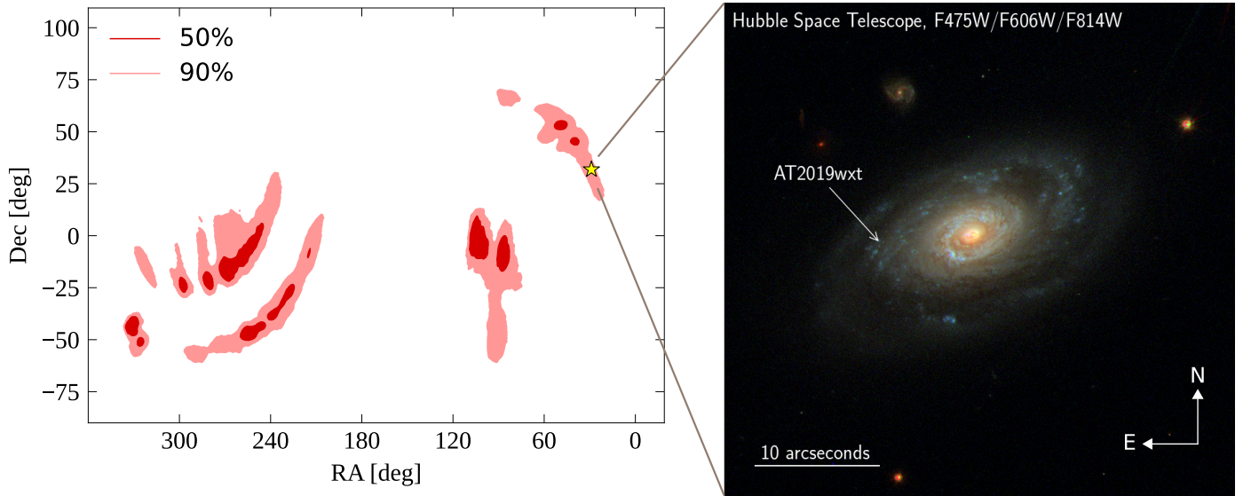
Fig. 1. SN 2019wxt localisation. Left-hand panel: Cartesian projection of the sky localisation error box of S191213g (50% and 90% localisation uncertainty contours – red and pink filled contours, respectively) compared to the position of SN 2019wxt (yellow star). The transient is located within the 90% localisation uncertainty contour. The GW localisation is based on the real-time parameter estimation reported in LVC (2019b). Right-hand panel: Colour composite HST image for SN 2019wxt and its host galaxy KUG 0152+311.
