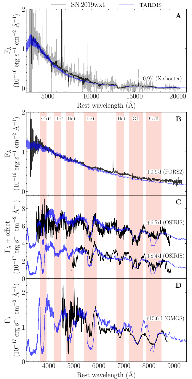
Fig. 8. Comparisons between our model spectra (blue) and observations (black). The observed spectra have been rebinned by a factor of 10 (using SPECTRES, Carnall 2017). Panel A: Comparison of the +0.9 d X-shooter spectrum with our best-fitting TARDIS model. Panel B: Comparison of the early FORS2 spectrum (+0.9 d), and our best-fitting TARDIS model. Panel C: Comparison of the two later OSIRIS spectra (+6.5 and +8.4 d) with their corresponding TARDIS models. The +6.5 d spectrum and model have been offset by 3 \times 10^{-17} \text{ erg s}^{-1} \text{ cm}^{-2} \text{ \AA}^{-1} , for clarity. Panel D: Comparison of the late-time GMOS spectrum (+15.6 d), and its corresponding TARDIS model. The vertical shaded bands in panels B, C and D correspond to regions of absorption in the observed spectra. The species dominating these same absorption features in our best-fitting TARDIS models have added to the top of each band in panel B.
