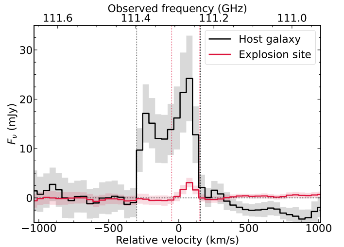
Fig. 13. CO spectra extracted over the entire SN host galaxy (black) and of the explosion site (red). The vertical dotted lines denote the spectral region from which the fluxes were extracted.
