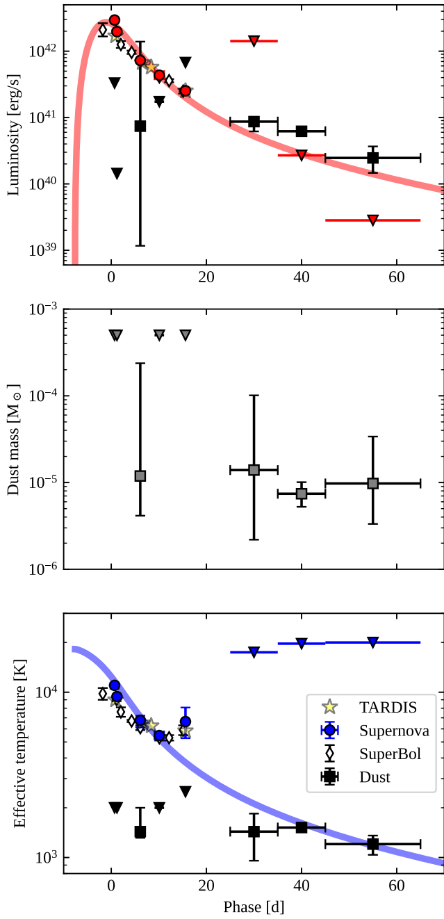
Fig. D.2. Evolution of SN luminosity, dust mass and effective temperatures from SED fitting. Red circles represent the blackbody (i.e. SN) while the black squares represent the modified blackbody (i.e. dust) luminosity (upper panel) and effective temperature. Downward-pointing triangles represent 3-sigma upper limits. Error bars show 90% credible intervals.
