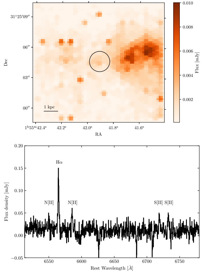
Fig. 10. Integral field spectroscopy of the host galaxy. Upper panel: H \alpha map constructed from 2D MEGARA+LR-R spectrum. The aperture used to extract the host galaxy spectrum is indicated with a black circle. Lower panel: MEGARA LR-R spectrum at the position of SN 2019wxt showing detected host galaxy lines.
