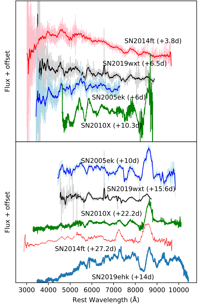
Fig. 15. Spectral comparison of SN 2019wxt at +6.5 d (upper panel) and +15.6 d (lower panel) to a sample of ultra-stripped SNe at similar phases. Low S/N spectra have been smoothed with a Savitzky-Golay filter (with a 100 \text{ \AA} window) for presentation purposes. We also show the possible Type IIb ultra-stripped SN 2019ehk in the lower panel. The flat topped line at \sim 6500 \text{ \AA} that has been suggested to be \text{H}\alpha (De et al. 2021) is either much weaker or absent in SN 2019wxt.
