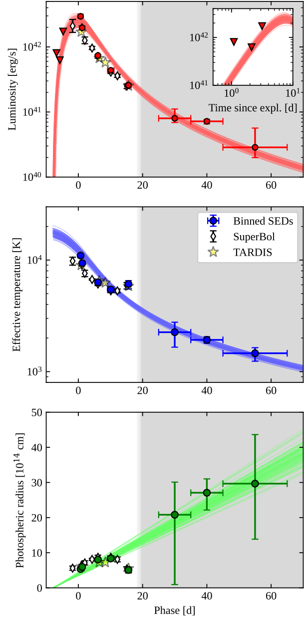
Fig. 9. Evolution of photospheric quantities from blackbody fits to photometric data. The figure shows the luminosity (top panel), effective temperature (middle panel) and photospheric radius (bottom panel) derived from fitting a blackbody spectrum to our photometric data at various epochs (circles with error bars show results from MCMC fitting of binned SEDs; white diamonds show the SuperBol bolometric fit results; star symbols show the results from our TARDIS model – Sect. 4.4). Thin lines are 100 posterior samples from our simple SN model (Appendix C) fitted to the photometric dataset. The grey shaded area corresponds to times when the ejecta are formally optically thin (nebular phase). The inset in the top panel shows the model samples plotted against the time since explosion, with a logarithmic x-axis to better display the agreement with the upper limits. The latter are derived from our z-band upper limits assuming the blackbody spectrum corresponding to the best-fit model.
