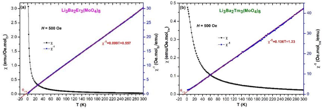
Figure 7 The dc susceptibility ( \chi ) and its inverse ( \chi^{-1} ) at constant field vs. temperature for \text{Li}_3\text{Ba}_2\text{Ln}_3(\text{MoO}_4)_8 showing a Curie-Weiss behavior (red line). \text{Ln} = \text{Er} (a); \text{Ln} = \text{Tm} (b)
