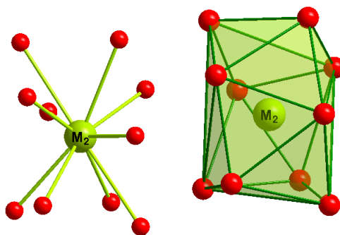
Figure 4 Oxygen environment and coordination polyhedron around the position M2
